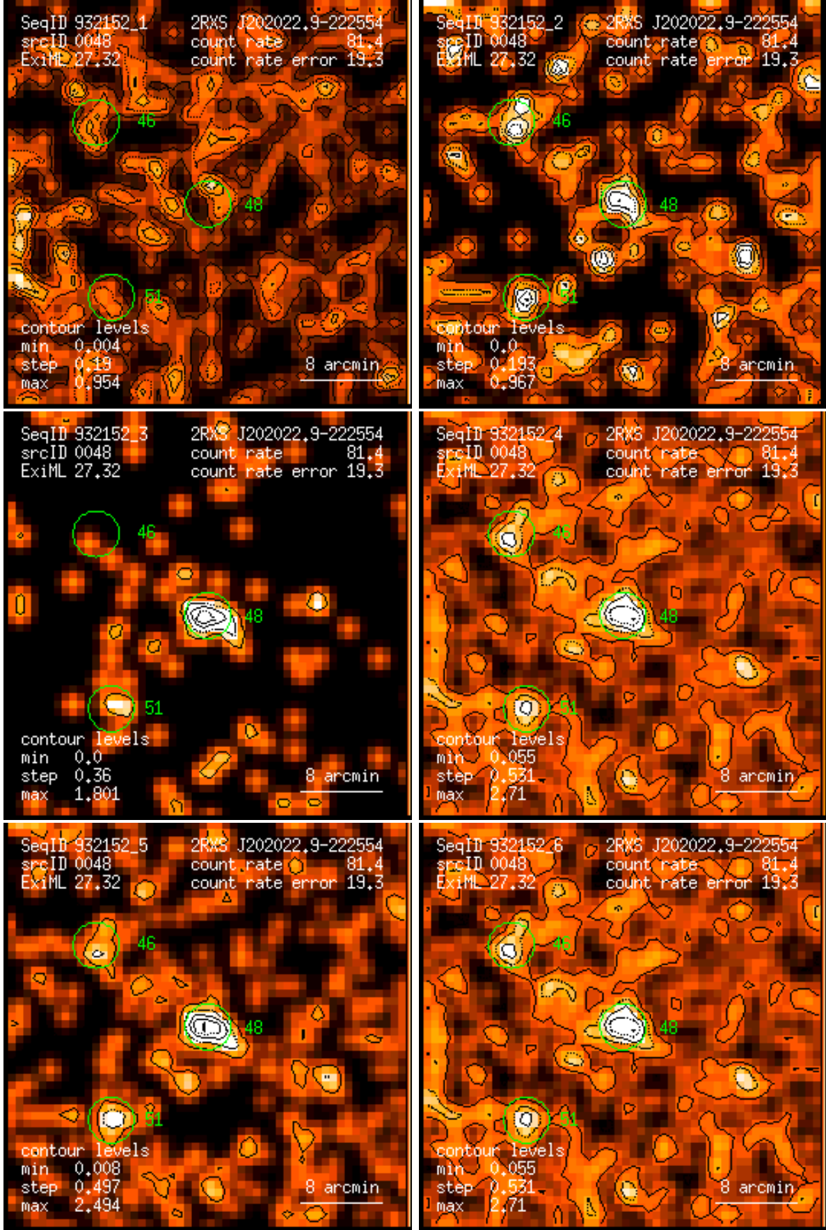
Figure 48: RASS 932152: detection 0048: band rate images, Gaussian filter: (1) PSPC channels 11 – 41, (2) 52 – 90, (3) 91 – 201, (4) 11 – 235, (5) 52 – 201, (6) 11 – 201. Broad band rates in counts/ks. Band rate contour levels in counts/ks/arcmin 2 .
