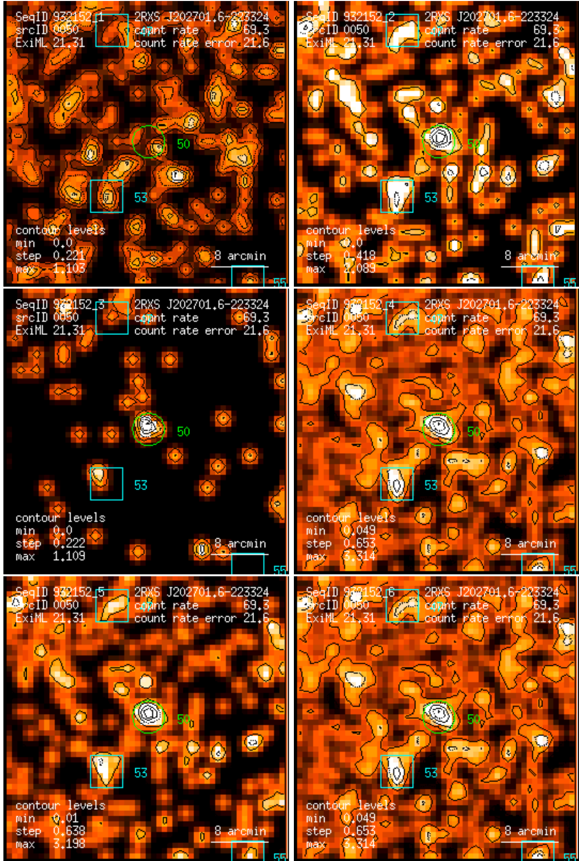
Figure 50: RASS 932152: detection 0050: band rate images, Gaussian filter: (1) PSPC channels 11 – 41, (2) 52 – 90, (3) 91 – 201, (4) 11 – 235, (5) 52 – 201, (6) 11 – 201. Broad band rates in counts/ks. Band rate contour levels in counts/ks/arcmin 2 .
