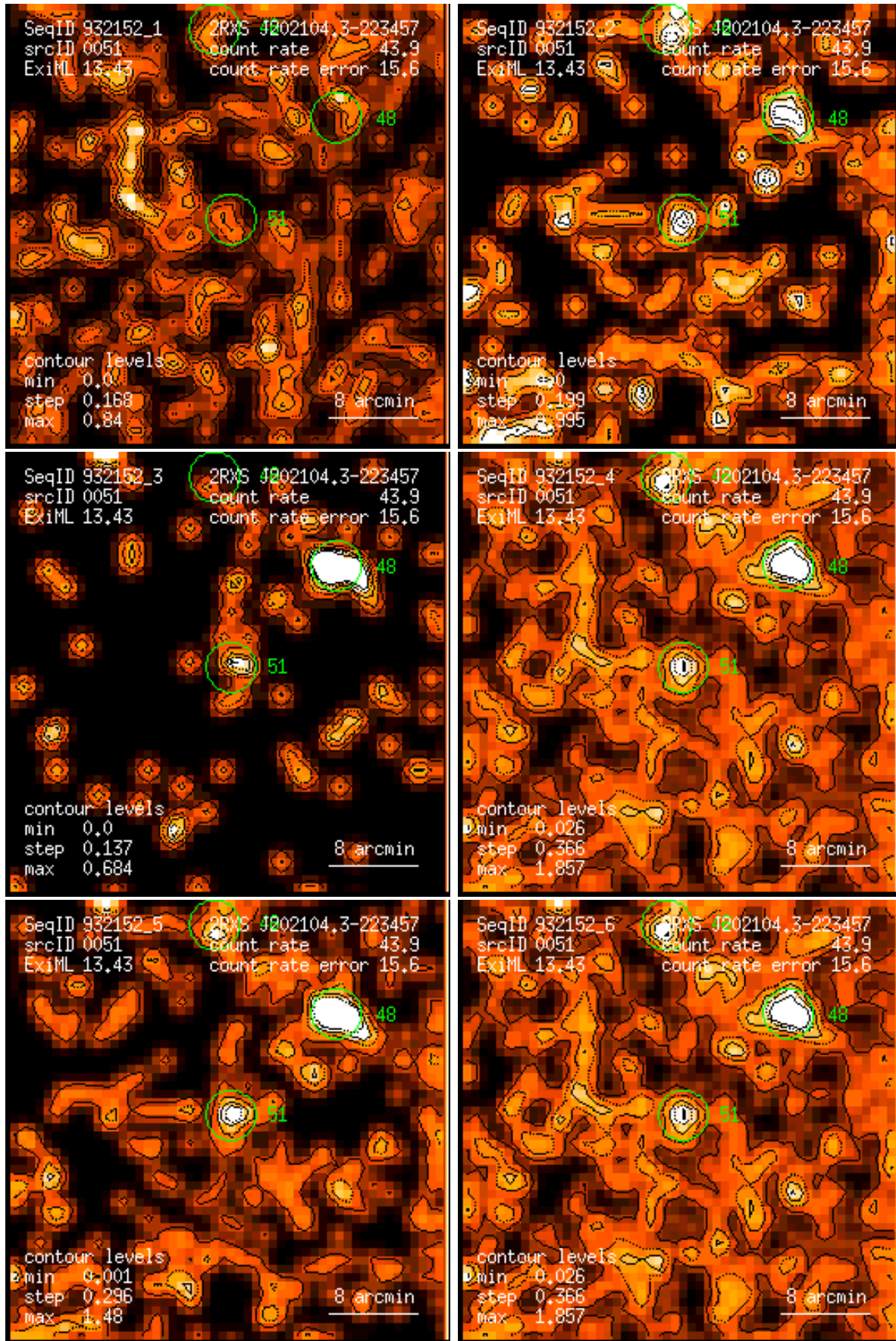
Figure 51: RASS 932152: detection 0051: band rate images, Gaussian filter: (1) PSPC channels 11 – 41, (2) 52 – 90, (3) 91 – 201, (4) 11 – 235, (5) 52 – 201, (6) 11 – 201. Broad band rates in counts/ks. Band rate contour levels in counts/ks/arcmin 2 .
