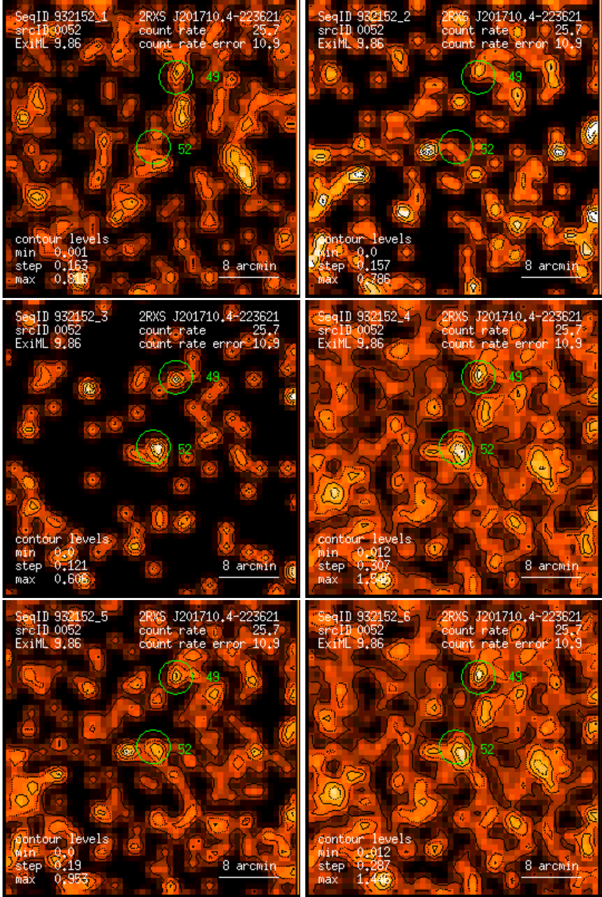
Figure 52: RASS 932152: detection 0052: band rate images, Gaussian filter: (1) PSPC channels 11 – 41, (2) 52 – 90, (3) 91 – 201, (4) 11 – 235, (5) 52 – 201, (6) 11 – 201. Broad band rates in counts/ks. Band rate contour levels in counts/ks/arcmin 2 .
