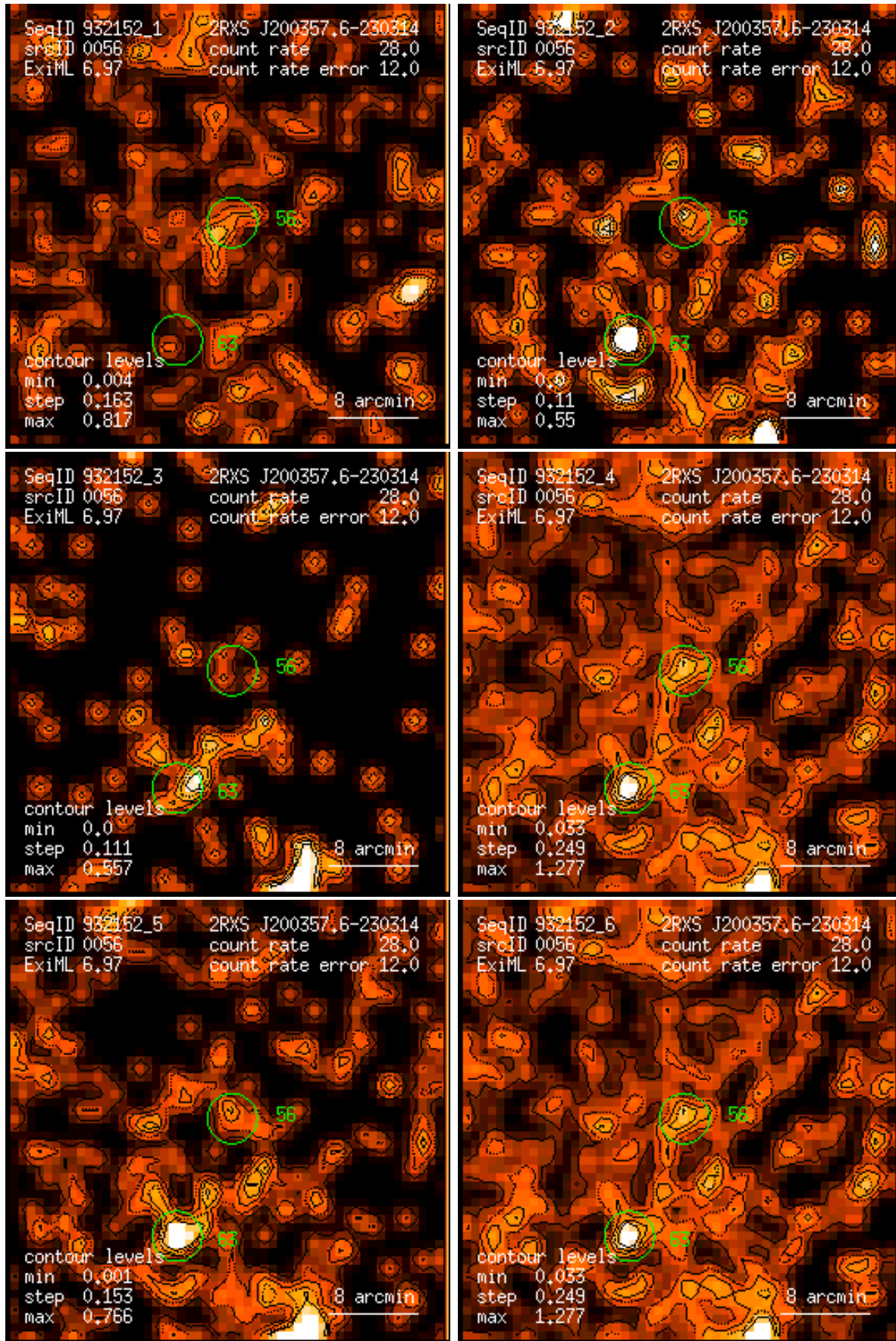
Figure 56: RASS 932152: detection 0056: band rate images, Gaussian filter: (1) PSPC channels 11 – 41, (2) 52 – 90, (3) 91 – 201, (4) 11 – 235, (5) 52 – 201, (6) 11 – 201. Broad band rates in counts/ks. Band rate contour levels in counts/ks/arcmin 2 .
