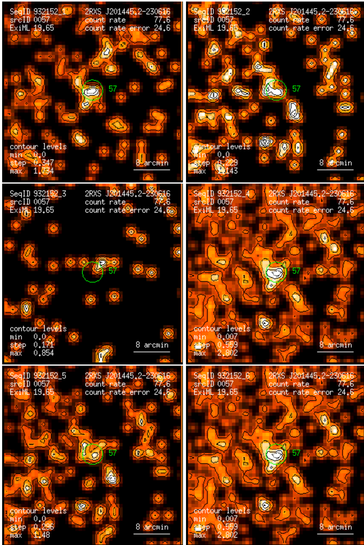
Figure 57: RASS 932152: detection 0057: band rate images, Gaussian filter: (1) PSPC channels 11 – 41, (2) 52 – 90, (3) 91 – 201, (4) 11 – 235, (5) 52 – 201, (6) 11 – 201. Broad band rates in counts/ks. Band rate contour levels in counts/ks/arcmin 2 .
