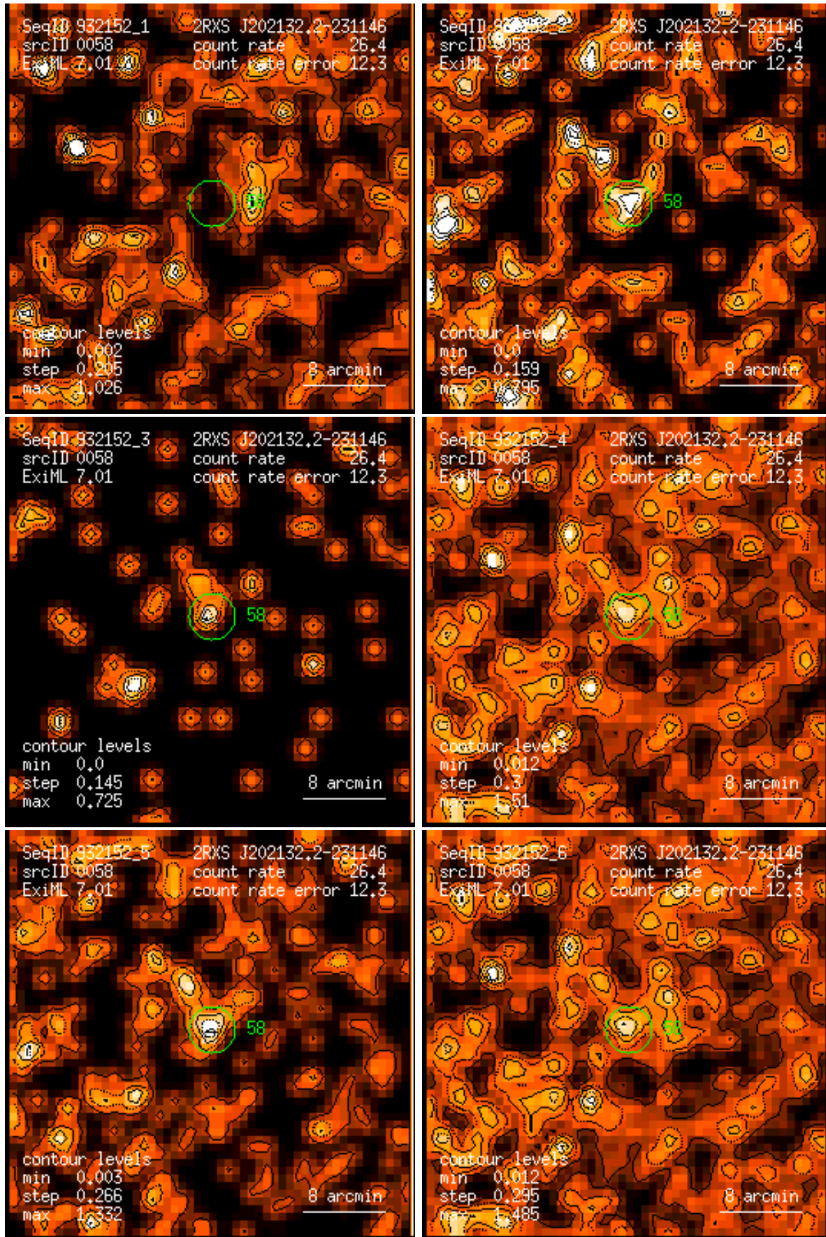
Figure 58: RASS 932152: detection 0058: band rate images, Gaussian filter: (1) PSPC channels 11 – 41, (2) 52 – 90, (3) 91 – 201, (4) 11 – 235, (5) 52 – 201, (6) 11 – 201. Broad band rates in counts/ks. Band rate contour levels in counts/ks/arcmin 2 .
