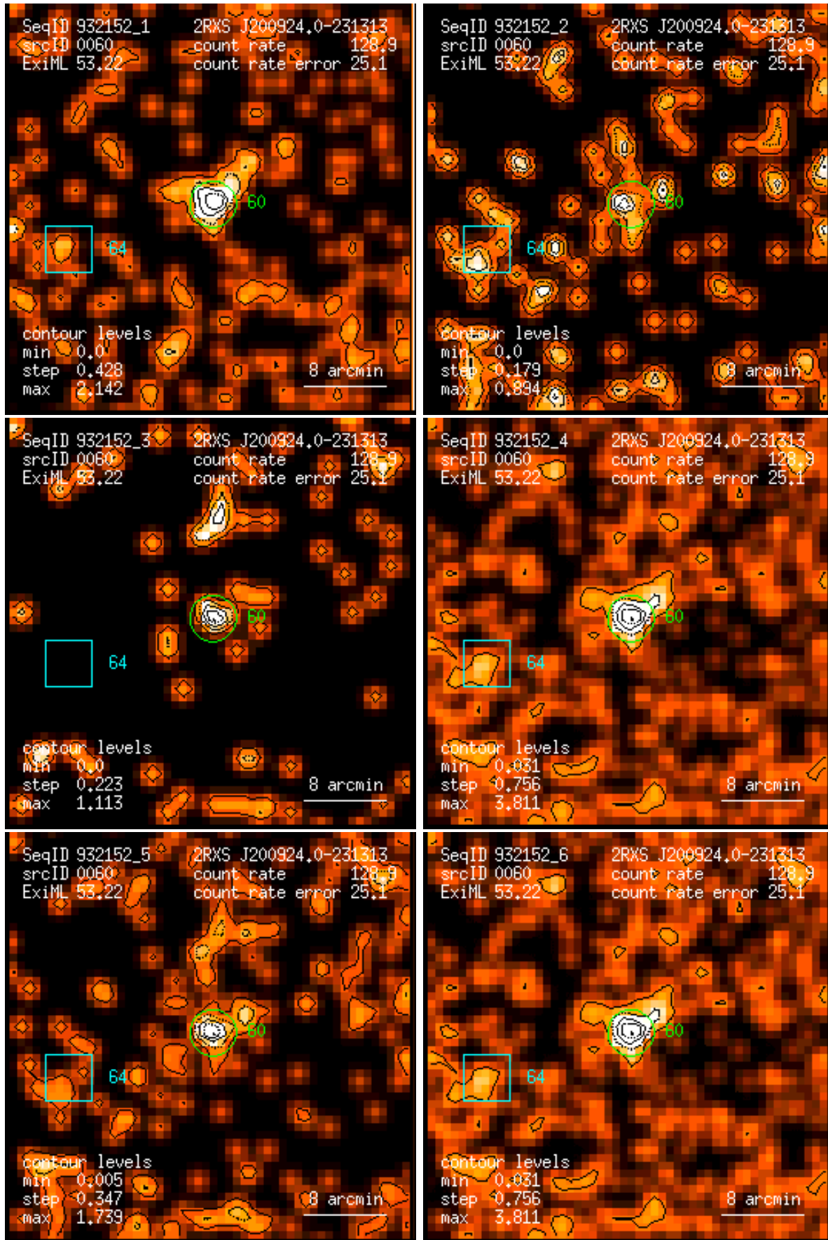
Figure 60: RASS 932152: detection 0060: band rate images, Gaussian filter: (1) PSPC channels 11 – 41, (2) 52 – 90, (3) 91 – 201, (4) 11 – 235, (5) 52 – 201, (6) 11 – 201. Broad band rates in counts/ks. Band rate contour levels in counts/ks/arcmin 2 .
