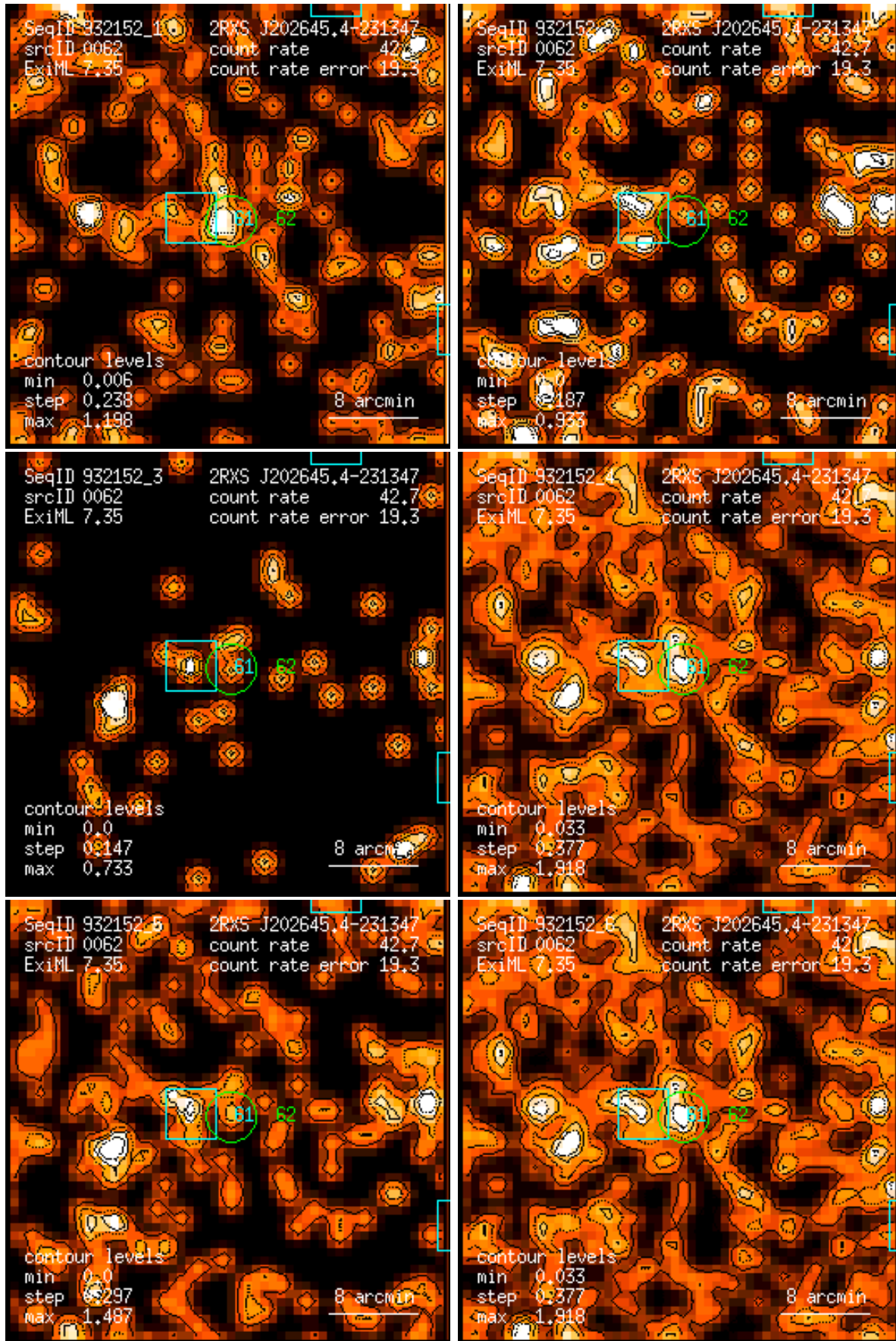
Figure 62: RASS 932152: detection 0062: band rate images, Gaussian filter: (1) PSPC channels 11 – 41, (2) 52 – 90, (3) 91 – 201, (4) 11 – 235, (5) 52 – 201, (6) 11 – 201. Broad band rates in counts/ks. Band rate contour levels in counts/ks/arcmin 2 .
