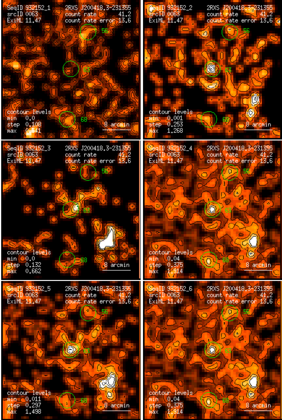
Figure 63: RASS 932152: detection 0063: band rate images, Gaussian filter: (1) PSPC channels 11 – 41, (2) 52 – 90, (3) 91 – 201, (4) 11 – 235, (5) 52 – 201, (6) 11 – 201. Broad band rates in counts/ks. Band rate contour levels in counts/ks/arcmin 2 .
