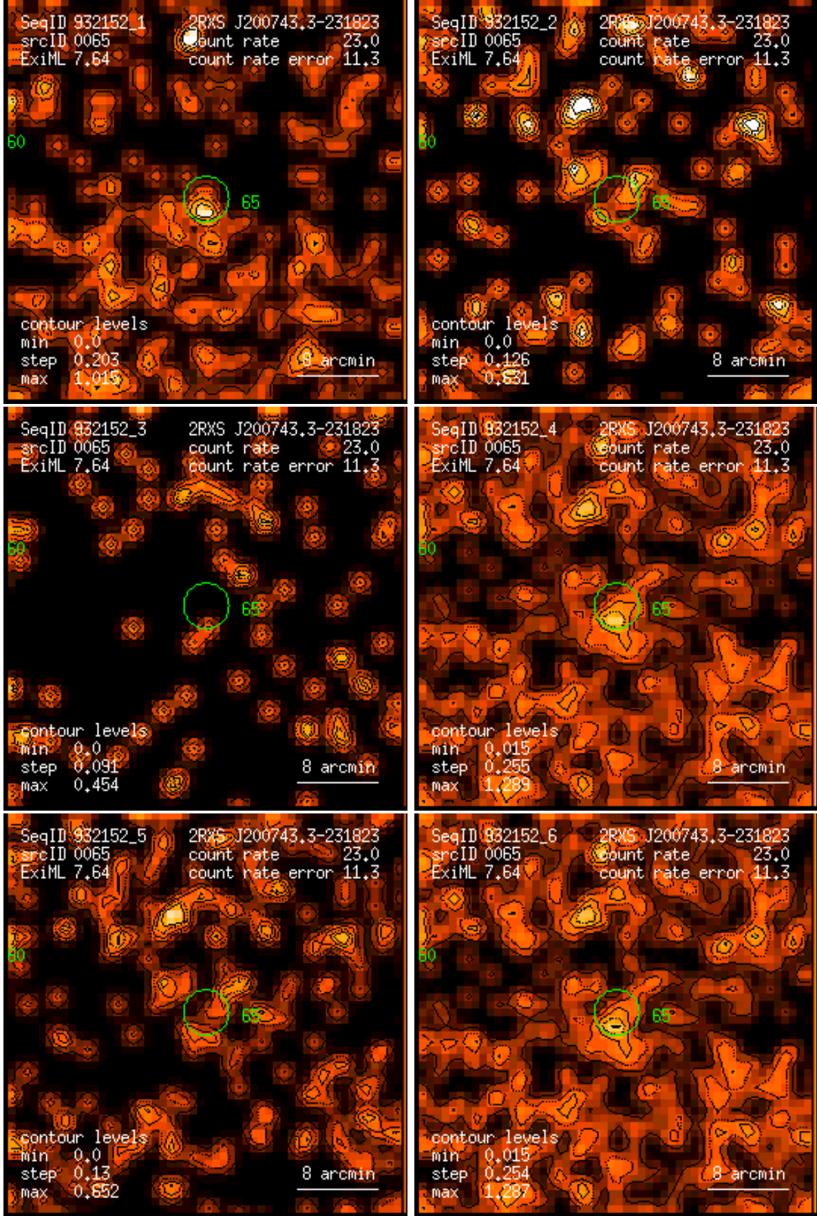
Figure 65: RASS 932152: detection 0065: band rate images, Gaussian filter: (1) PSPC channels 11 – 41, (2) 52 – 90, (3) 91 – 201, (4) 11 – 235, (5) 52 – 201, (6) 11 – 201. Broad band rates in counts/ks. Band rate contour levels in counts/ks/arcmin 2 .
