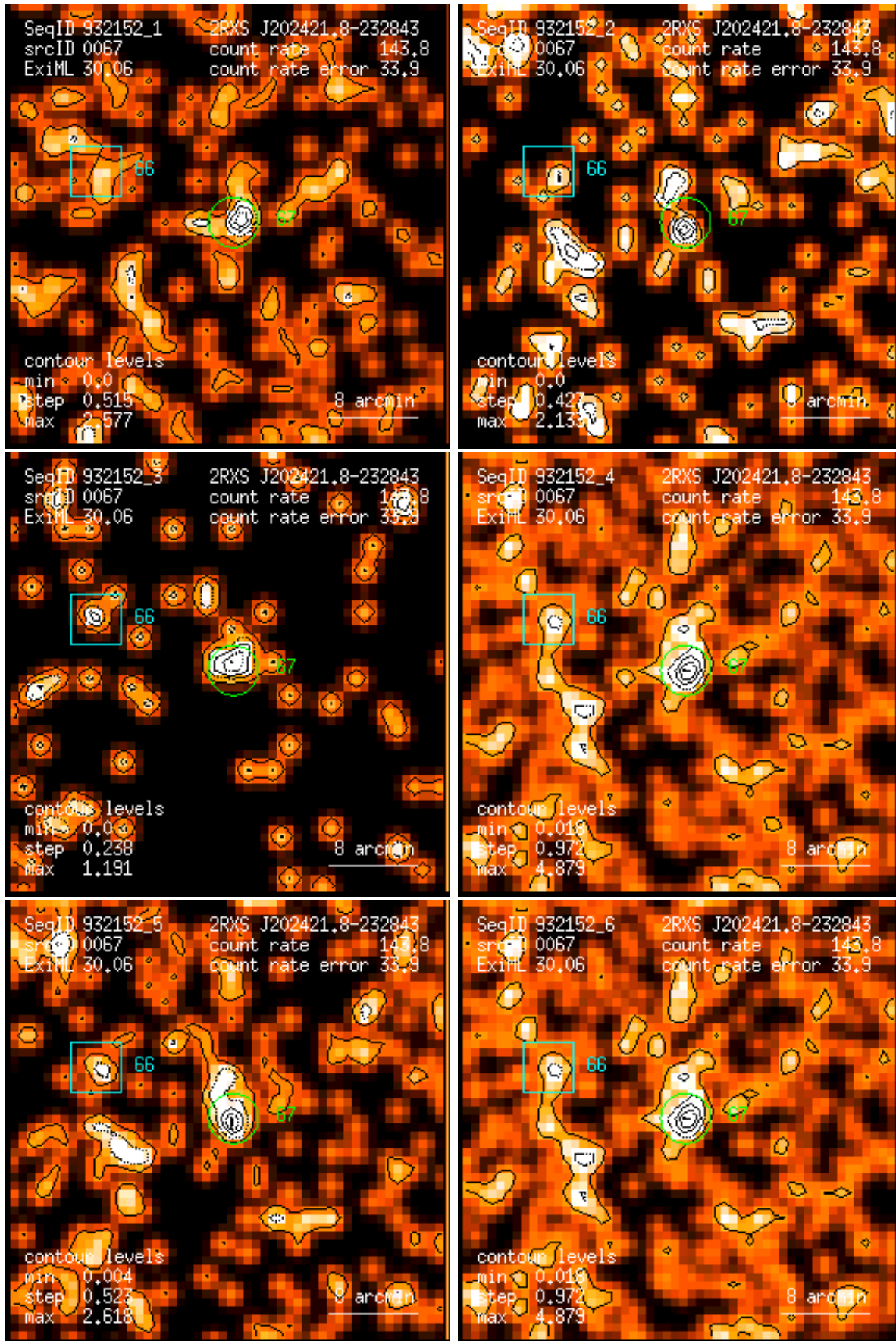
Figure 67: RASS 932152: detection 0067: band rate images, Gaussian filter: (1) PSPC channels 11 – 41, (2) 52 – 90, (3) 91 – 201, (4) 11 – 235, (5) 52 – 201, (6) 11 – 201. Broad band rates in counts/ks. Band rate contour levels in counts/ks/arcmin 2 .
