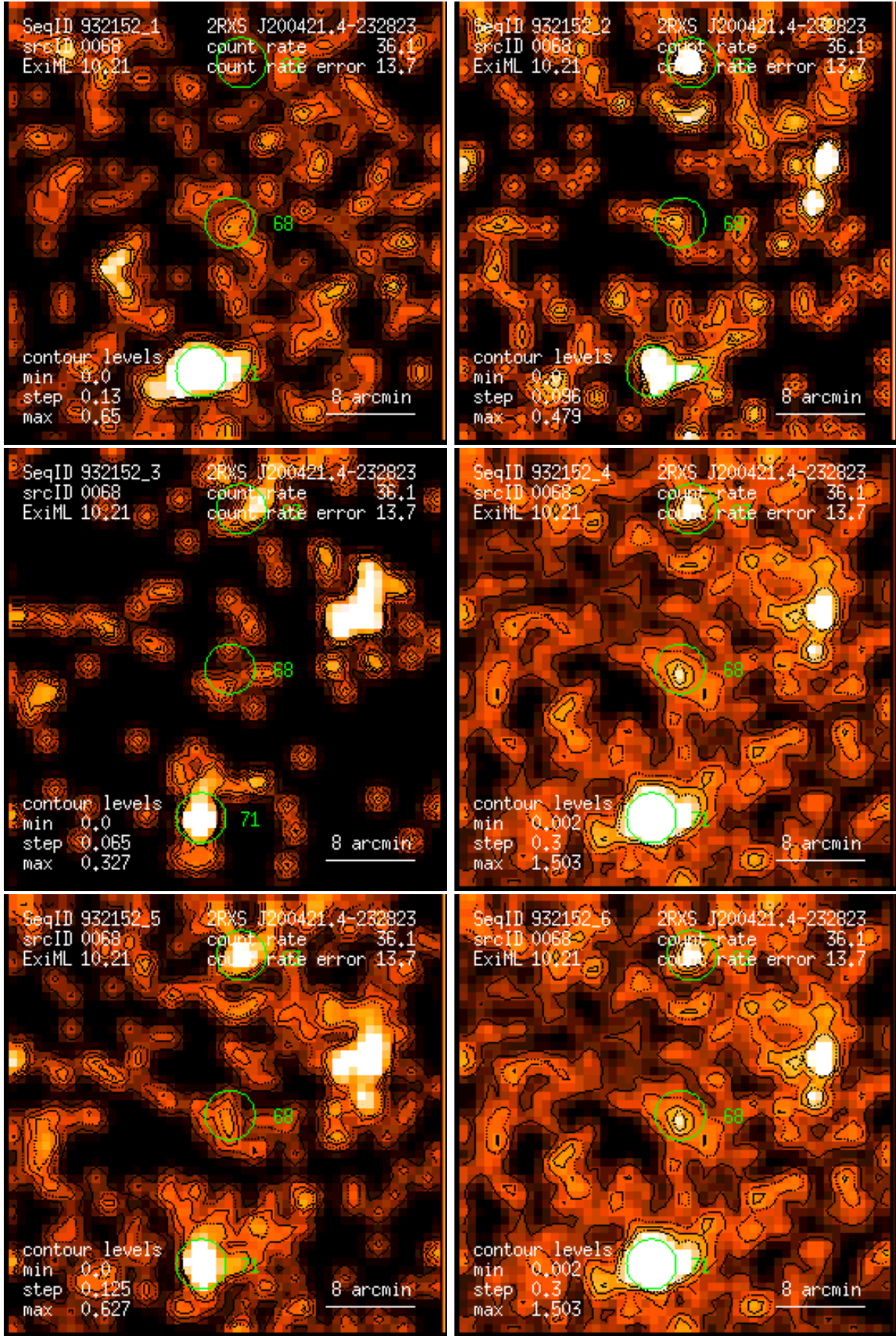
Figure 68: RASS 932152: detection 0068: band rate images, Gaussian filter: (1) PSPC channels 11 – 41, (2) 52 – 90, (3) 91 – 201, (4) 11 – 235, (5) 52 – 201, (6) 11 – 201. Broad band rates in counts/ks. Band rate contour levels in counts/ks/arcmin 2 .
