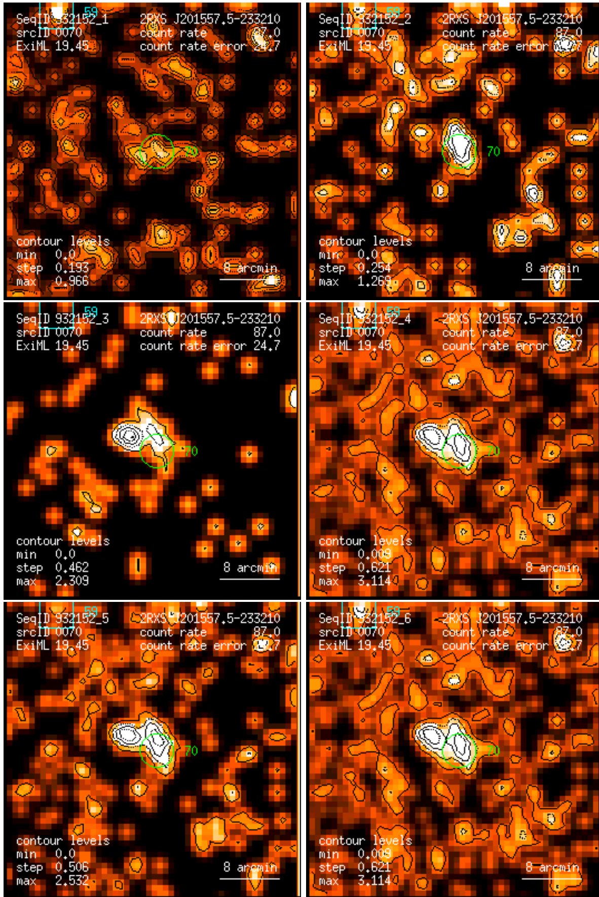
Figure 70: RASS 932152: detection 0070: band rate images, Gaussian filter: (1) PSPC channels 11 – 41, (2) 52 – 90, (3) 91 – 201, (4) 11 – 235, (5) 52 – 201, (6) 11 – 201. Broad band rates in counts/ks. Band rate contour levels in counts/ks/arcmin 2 .
