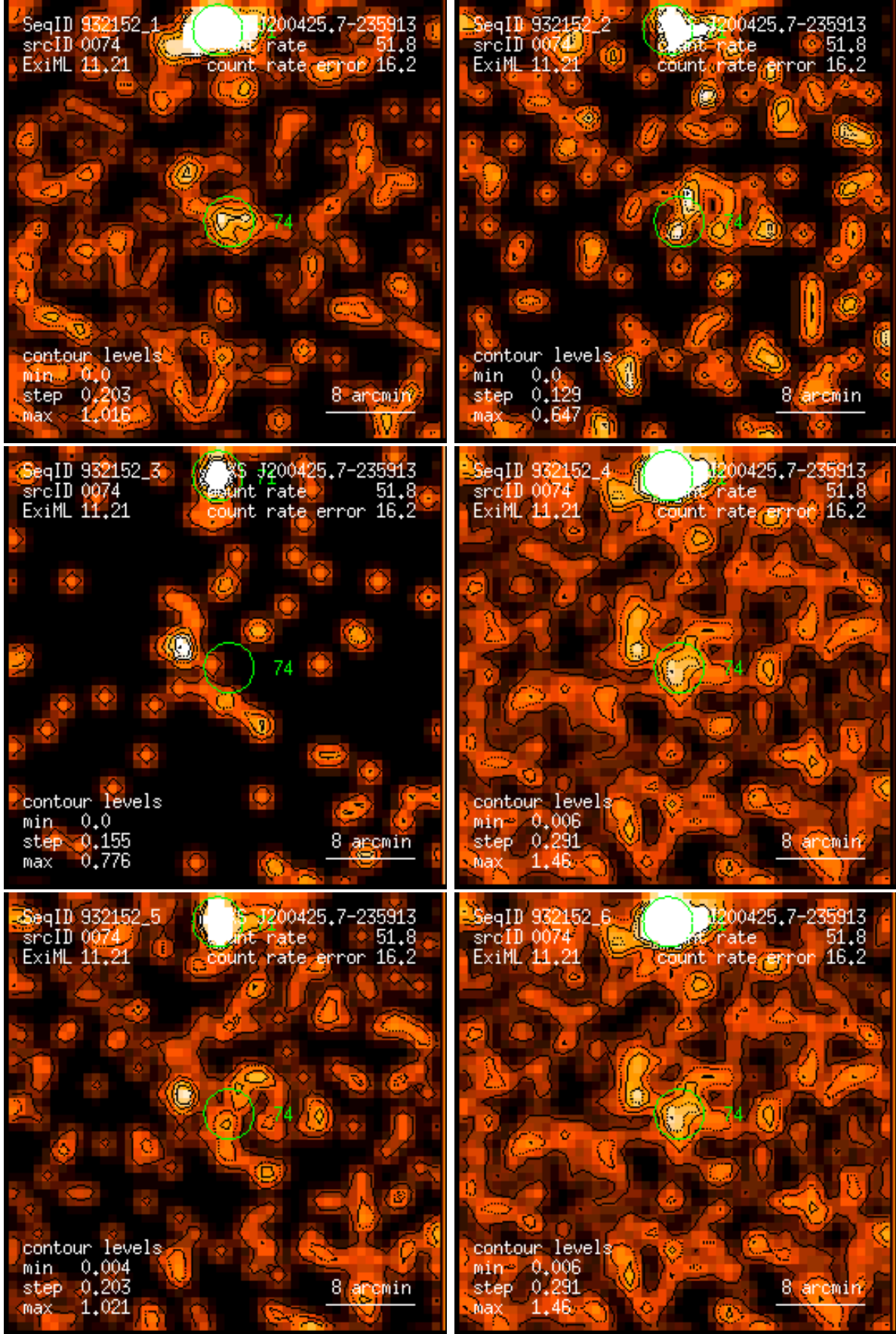
Figure 74: RASS 932152: detection 0074: band rate images, Gaussian filter: (1) PSPC channels 11 – 41, (2) 52 – 90, (3) 91 – 201, (4) 11 – 235, (5) 52 – 201, (6) 11 – 201. Broad band rates in counts/ks. Band rate contour levels in counts/ks/arcmin 2 .
