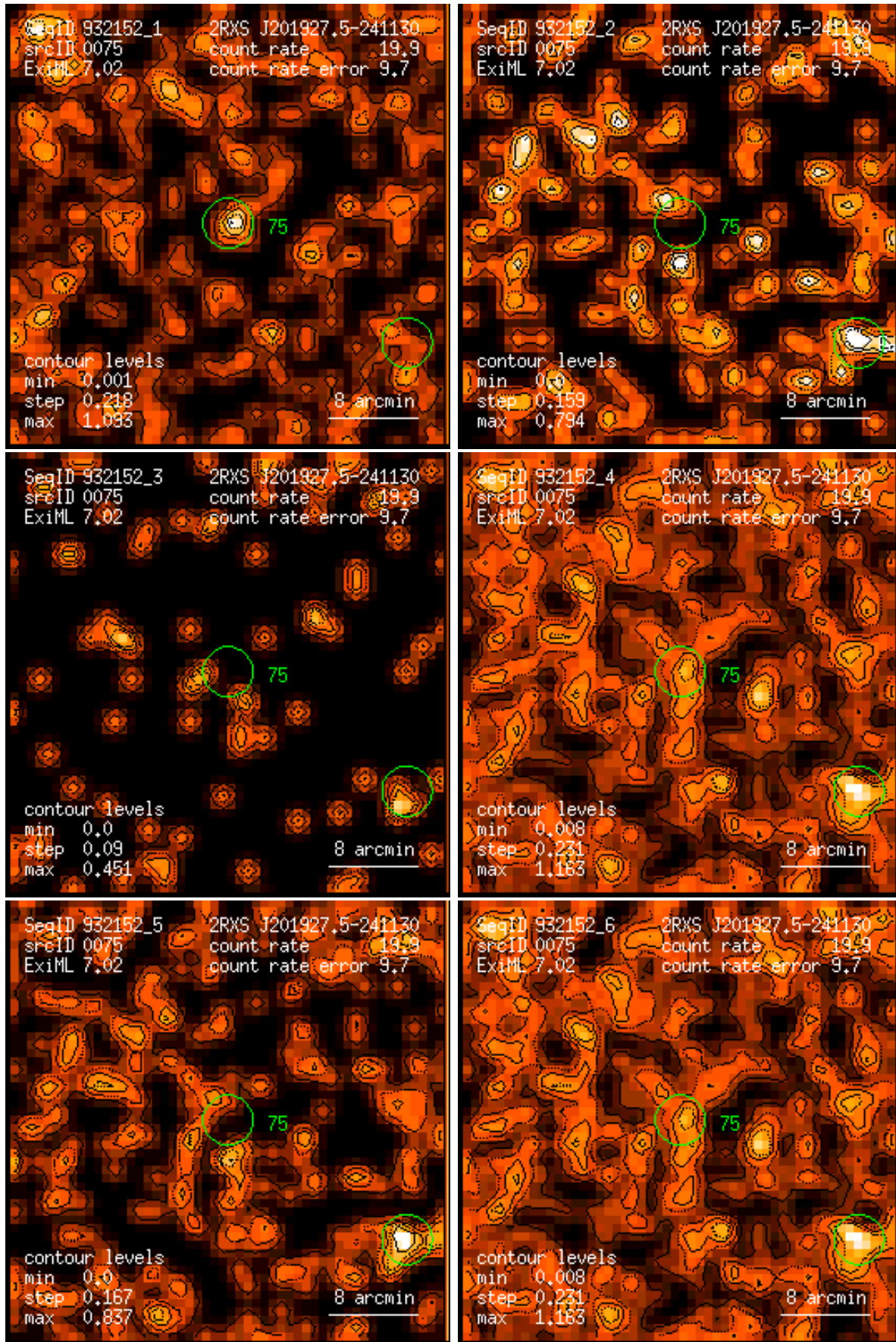
Figure 75: RASS 932152: detection 0075: band rate images, Gaussian filter: (1) PSPC channels 11 – 41, (2) 52 – 90, (3) 91 – 201, (4) 11 – 235, (5) 52 – 201, (6) 11 – 201. Broad band rates in counts/ks. Band rate contour levels in counts/ks/arcmin 2 .
