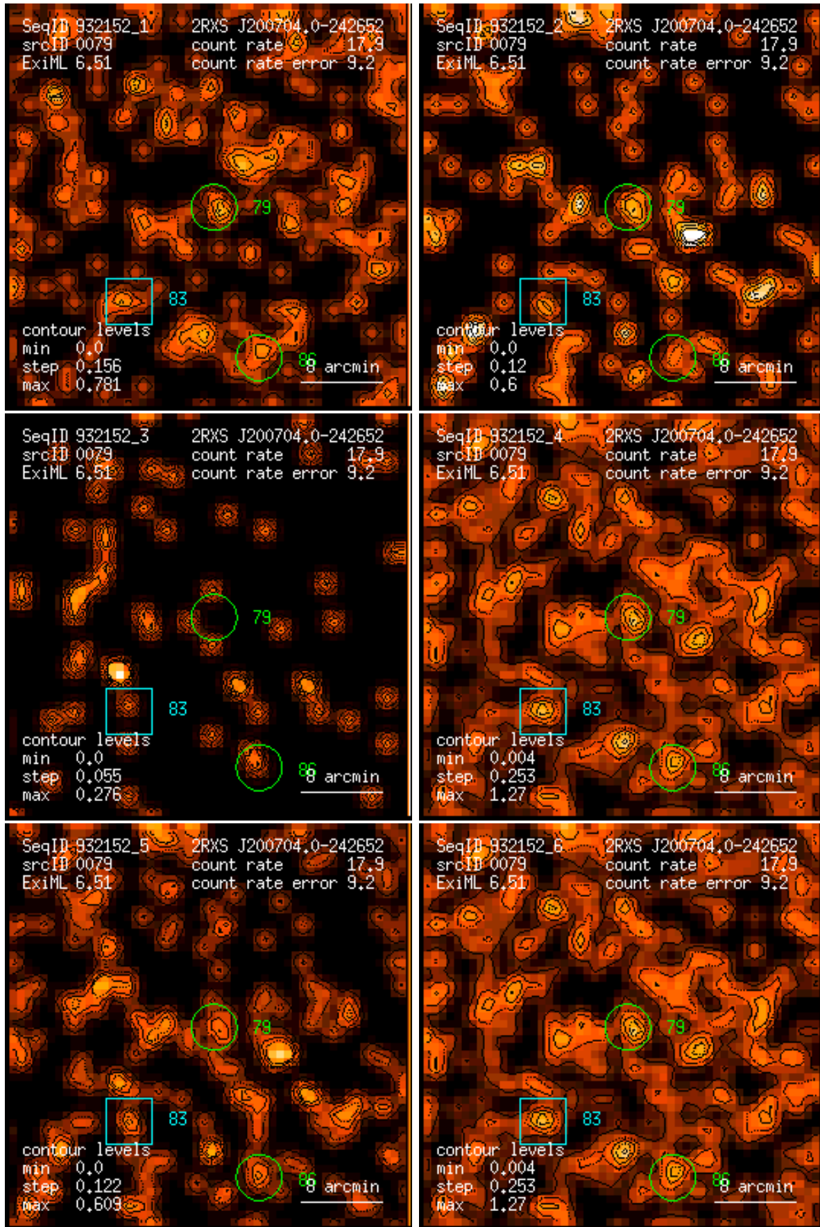
Figure 79: RASS 932152: detection 0079: band rate images, Gaussian filter: (1) PSPC channels 11 – 41, (2) 52 – 90, (3) 91 – 201, (4) 11 – 235, (5) 52 – 201, (6) 11 – 201. Broad band rates in counts/ks. Band rate contour levels in counts/ks/arcmin 2 .
