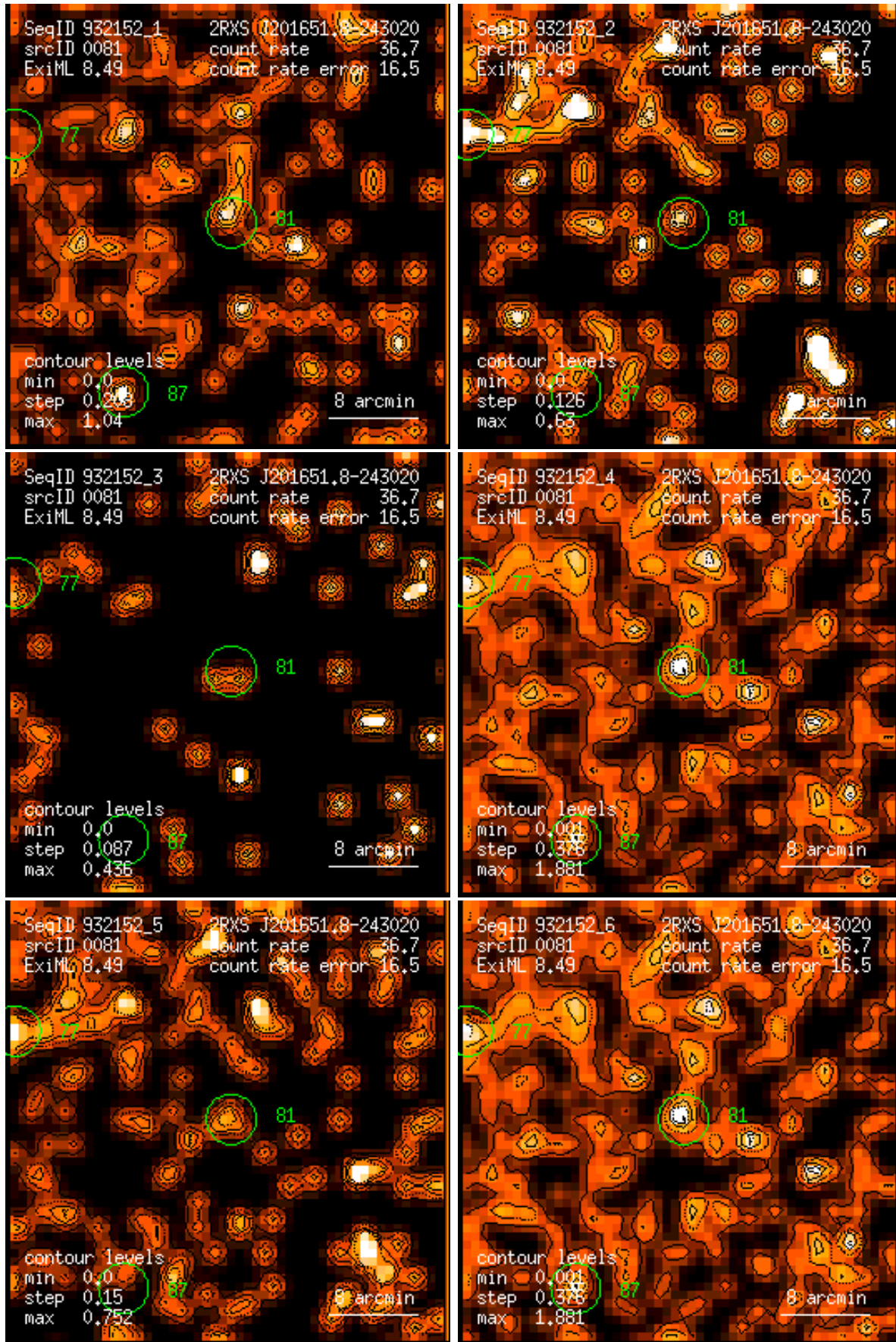
Figure 81: RASS 932152: detection 0081: band rate images, Gaussian filter: (1) PSPC channels 11 – 41, (2) 52 – 90, (3) 91 – 201, (4) 11 – 235, (5) 52 – 201, (6) 11 – 201. Broad band rates in counts/ks. Band rate contour levels in counts/ks/arcmin 2 .
