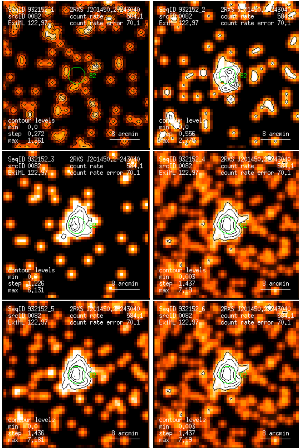
Figure 82: RASS 932152: detection 0082: band rate images, Gaussian filter: (1) PSPC channels 11 – 41, (2) 52 – 90, (3) 91 – 201, (4) 11 – 235, (5) 52 – 201, (6) 11 – 201. Broad band rates in counts/ks. Band rate contour levels in counts/ks/arcmin 2 .
