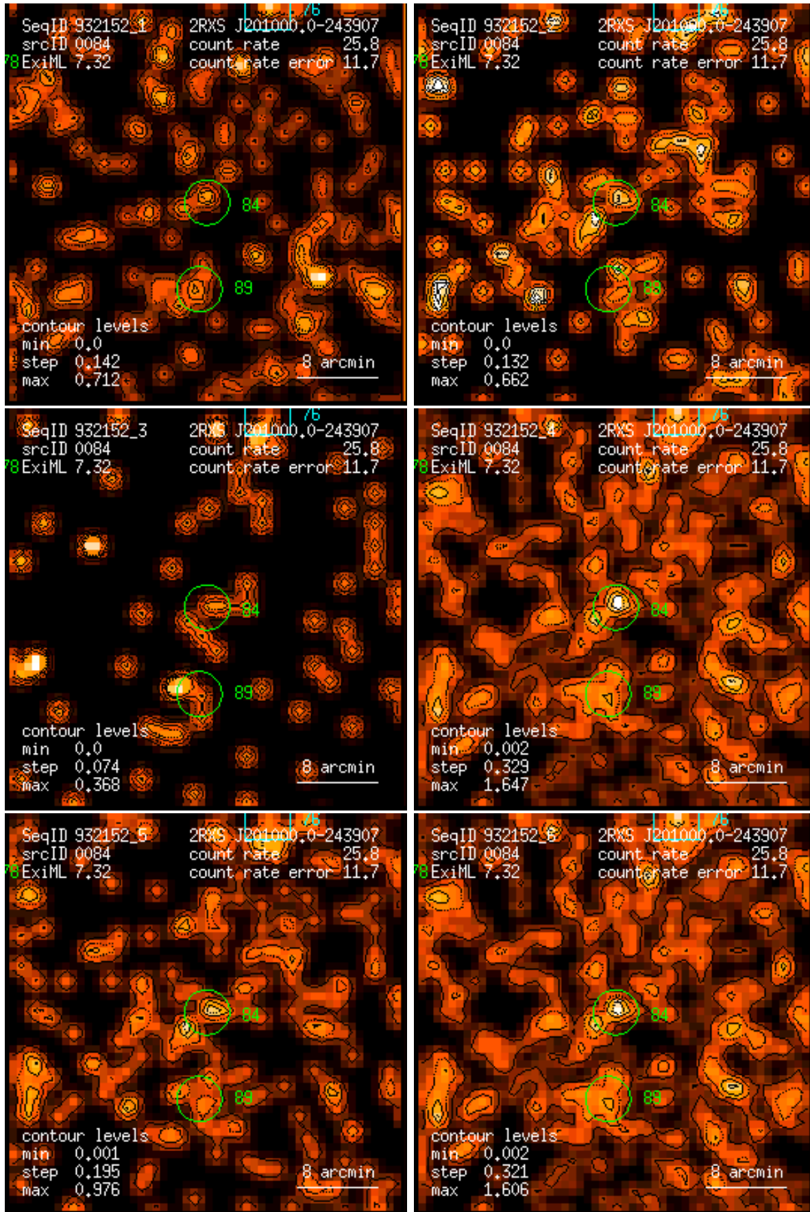
Figure 84: RASS 932152: detection 0084: band rate images, Gaussian filter: (1) PSPC channels 11 – 41, (2) 52 – 90, (3) 91 – 201, (4) 11 – 235, (5) 52 – 201, (6) 11 – 201. Broad band rates in counts/ks. Band rate contour levels in counts/ks/arcmin 2 .
