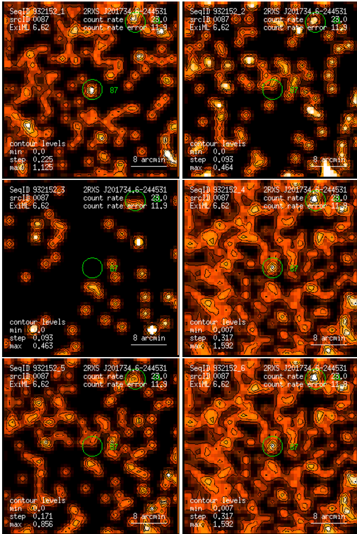
Figure 87: RASS 932152: detection 0087: band rate images, Gaussian filter: (1) PSPC channels 11 – 41, (2) 52 – 90, (3) 91 – 201, (4) 11 – 235, (5) 52 – 201, (6) 11 – 201. Broad band rates in counts/ks. Band rate contour levels in counts/ks/arcmin 2 .
