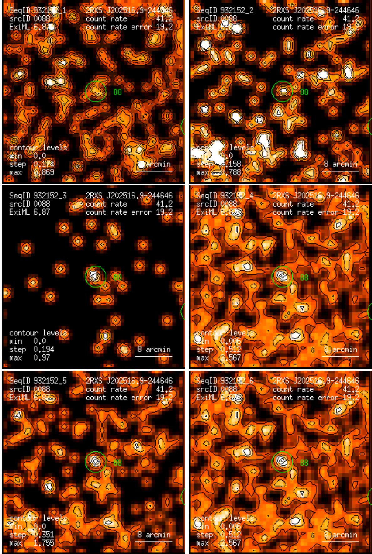
Figure 88: RASS 932152: detection 0088: band rate images, Gaussian filter: (1) PSPC channels 11 – 41, (2) 52 – 90, (3) 91 – 201, (4) 11 – 235, (5) 52 – 201, (6) 11 – 201. Broad band rates in counts/ks. Band rate contour levels in counts/ks/arcmin 2 .
