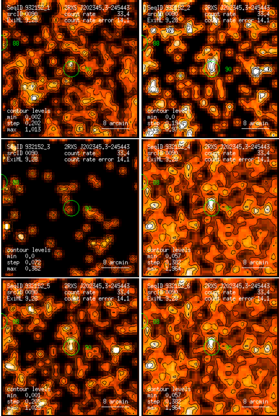
Figure 90: RASS 932152: detection 0090: band rate images, Gaussian filter: (1) PSPC channels 11 – 41, (2) 52 – 90, (3) 91 – 201, (4) 11 – 235, (5) 52 – 201, (6) 11 – 201. Broad band rates in counts/ks. Band rate contour levels in counts/ks/arcmin 2 .
