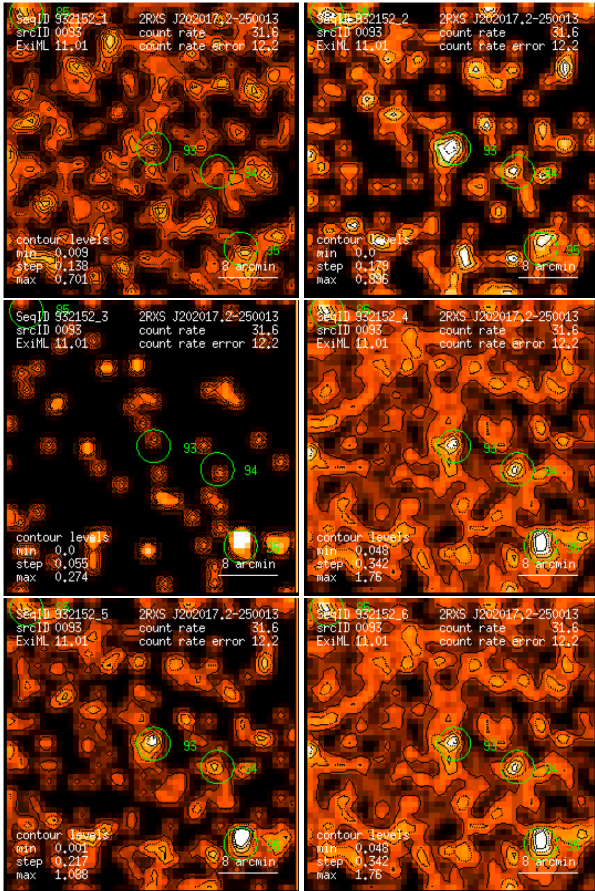
Figure 93: RASS 932152: detection 0093: band rate images, Gaussian filter: (1) PSPC channels 11 – 41, (2) 52 – 90, (3) 91 – 201, (4) 11 – 235, (5) 52 – 201, (6) 11 – 201. Broad band rates in counts/ks. Band rate contour levels in counts/ks/arcmin 2 .
