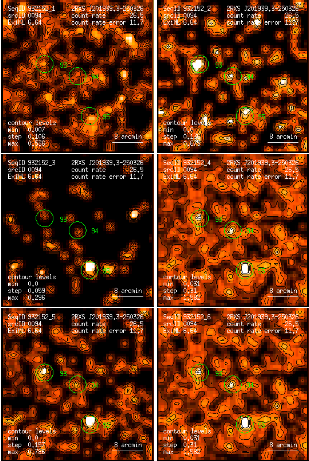
Figure 94: RASS 932152: detection 0094: band rate images, Gaussian filter: (1) PSPC channels 11 – 41, (2) 52 – 90, (3) 91 – 201, (4) 11 – 235, (5) 52 – 201, (6) 11 – 201. Broad band rates in counts/ks. Band rate contour levels in counts/ks/arcmin 2 .
