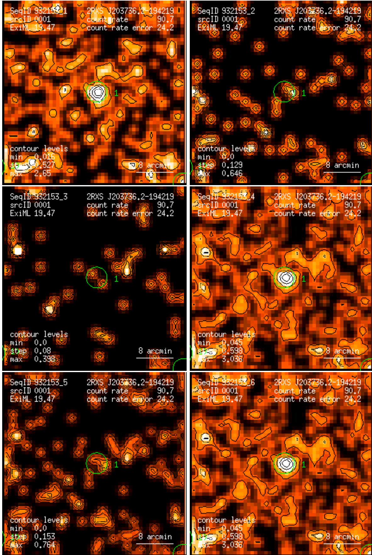
Figure 1: RASS 932153: detection 0001: band rate images, Gaussian filter: (1) PSPC channels 11 – 41, (2) 52 – 90, (3) 91 – 201, (4) 11 – 235, (5) 52 – 201, (6) 11 – 201. Broad band rates in counts/ks. Band rate contour levels in counts/ks/arcmin 2 .
