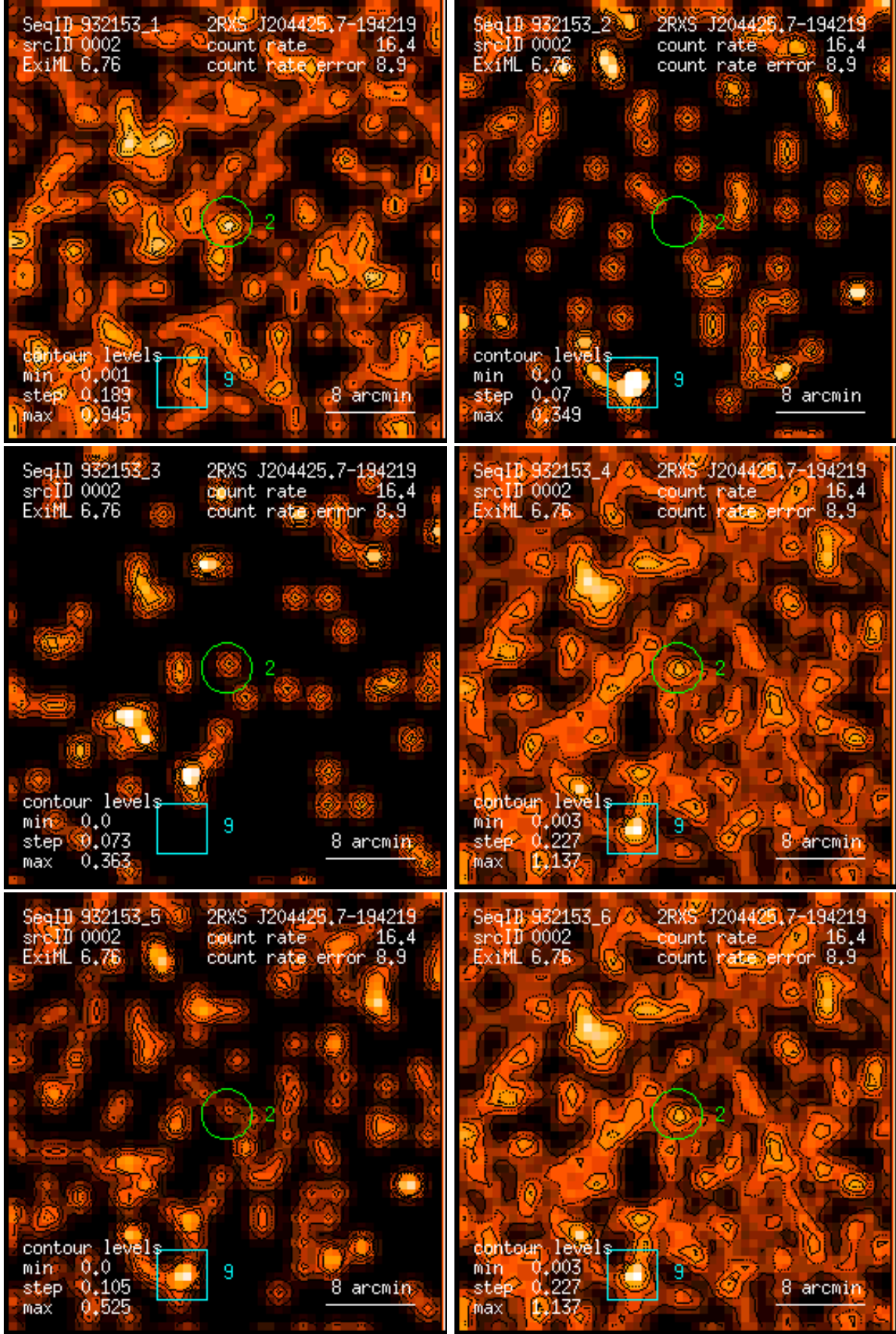
Figure 2: RASS 932153: detection 0002: band rate images, Gaussian filter: (1) PSPC channels 11 – 41, (2) 52 – 90, (3) 91 – 201, (4) 11 – 235, (5) 52 – 201, (6) 11 – 201. Broad band rates in counts/ks. Band rate contour levels in counts/ks/arcmin 2 .
