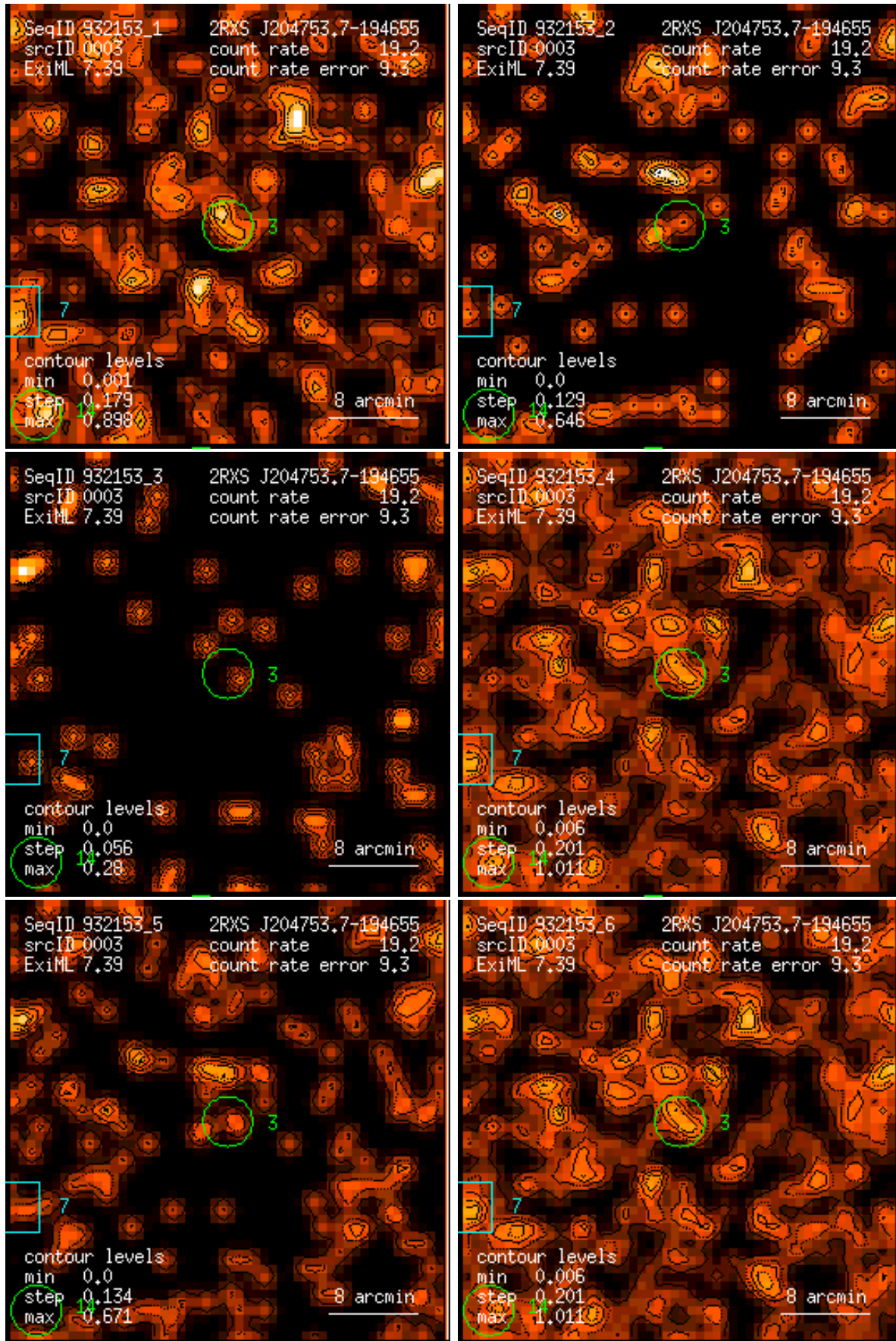
Figure 3: RASS 932153: detection 0003: band rate images, Gaussian filter: (1) PSPC channels 11 – 41, (2) 52 – 90, (3) 91 – 201, (4) 11 – 235, (5) 52 – 201, (6) 11 – 201. Broad band rates in counts/ks. Band rate contour levels in counts/ks/arcmin 2 .
