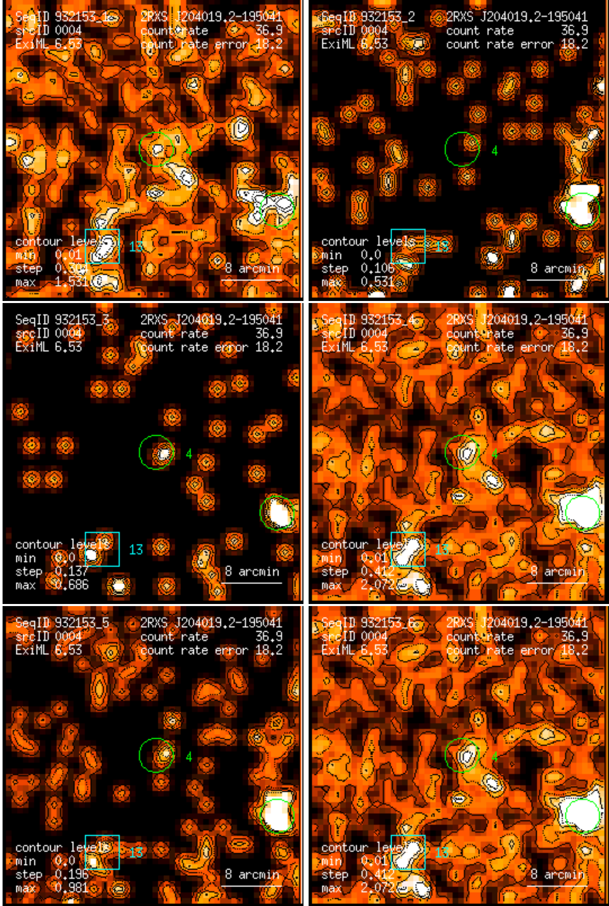
Figure 4: RASS 932153: detection 0004: band rate images, Gaussian filter: (1) PSPC channels 11 – 41, (2) 52 – 90, (3) 91 – 201, (4) 11 – 235, (5) 52 – 201, (6) 11 – 201. Broad band rates in counts/ks. Band rate contour levels in counts/ks/arcmin 2 .
