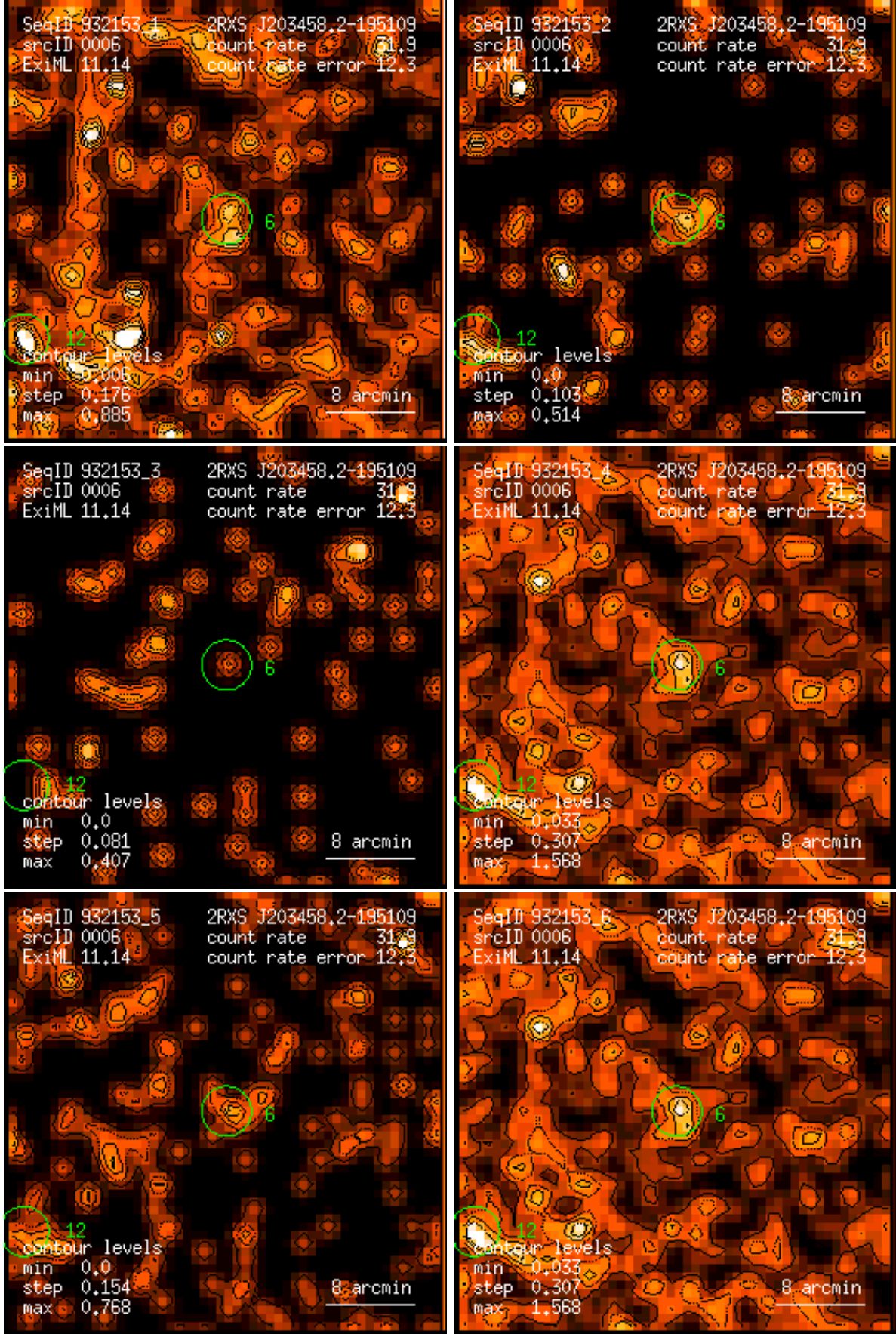
Figure 6: RASS 932153: detection 0006: band rate images, Gaussian filter: (1) PSPC channels 11 – 41, (2) 52 – 90, (3) 91 – 201, (4) 11 – 235, (5) 52 – 201, (6) 11 – 201. Broad band rates in counts/ks. Band rate contour levels in counts/ks/arcmin 2 .
