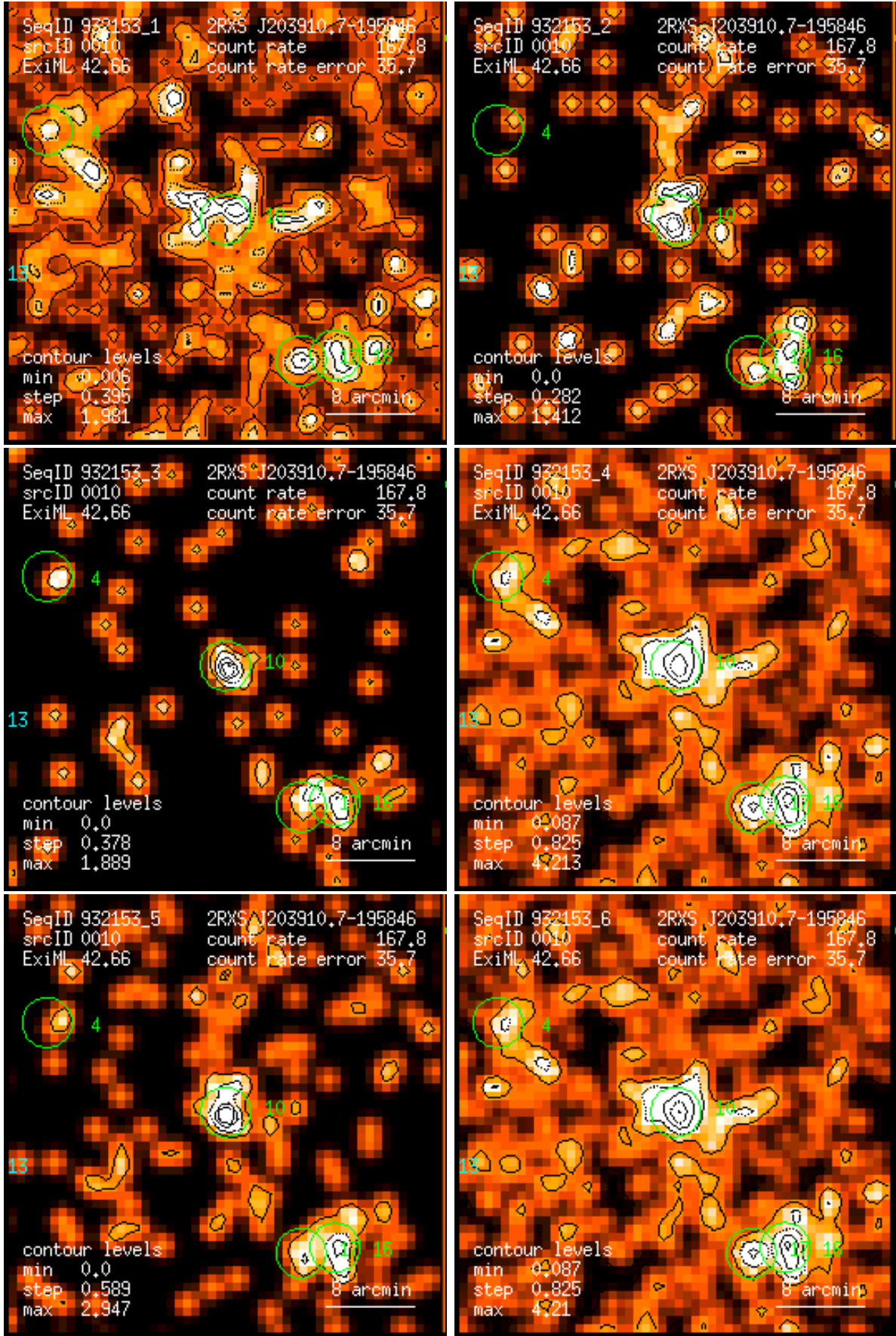
Figure 10: RASS 932153: detection 0010: band rate images, Gaussian filter: (1) PSPC channels 11 – 41, (2) 52 – 90, (3) 91 – 201, (4) 11 – 235, (5) 52 – 201, (6) 11 – 201. Broad band rates in counts/ks. Band rate contour levels in counts/ks/arcmin 2 .
