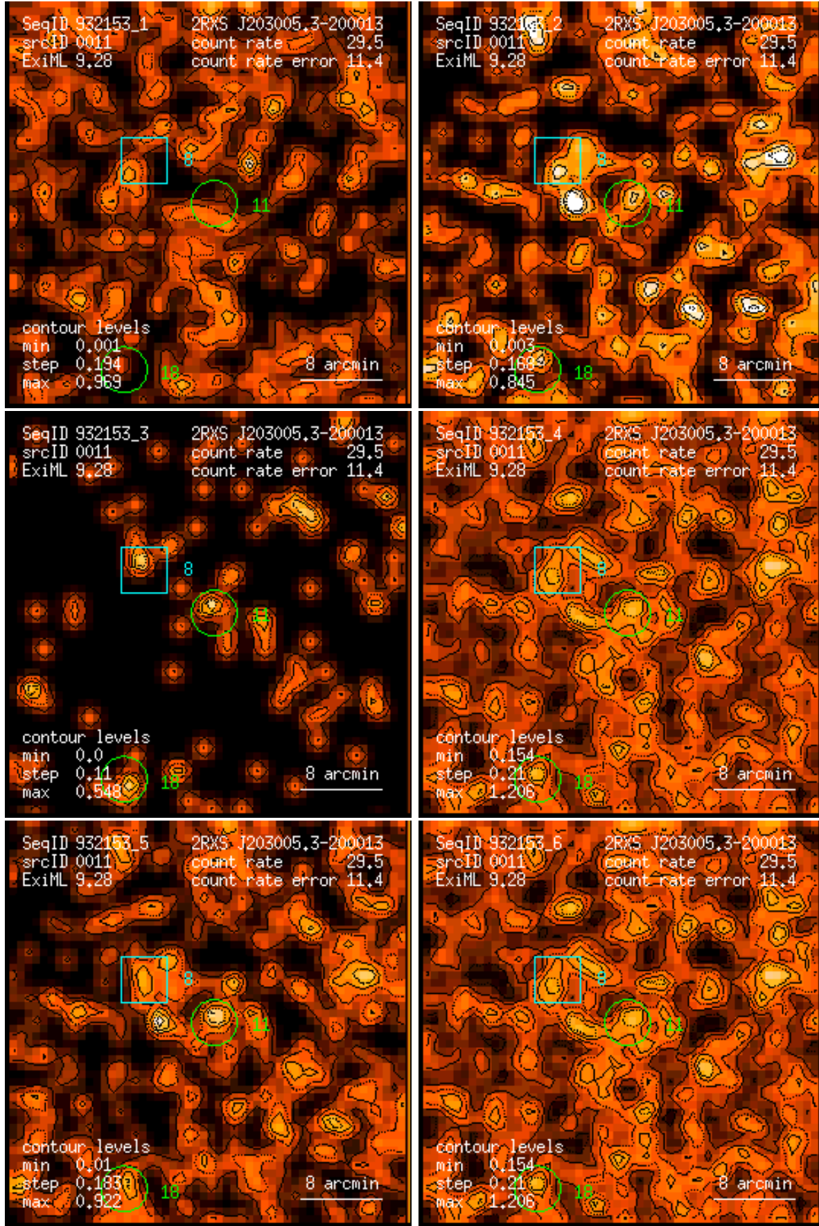
Figure 11: RASS 932153: detection 0011: band rate images, Gaussian filter: (1) PSPC channels 11 – 41, (2) 52 – 90, (3) 91 – 201, (4) 11 – 235, (5) 52 – 201, (6) 11 – 201. Broad band rates in counts/ks. Band rate contour levels in counts/ks/arcmin 2 .
