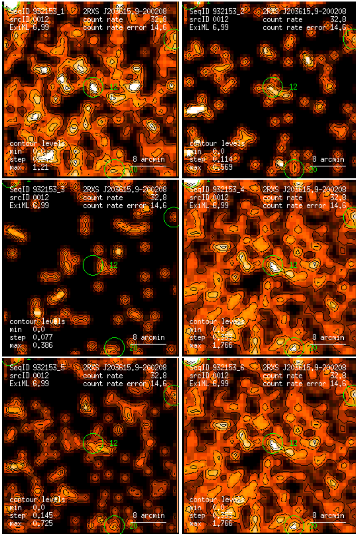
Figure 12: RASS 932153: detection 0012: band rate images, Gaussian filter: (1) PSPC channels 11 – 41, (2) 52 – 90, (3) 91 – 201, (4) 11 – 235, (5) 52 – 201, (6) 11 – 201. Broad band rates in counts/ks. Band rate contour levels in counts/ks/arcmin 2 .
