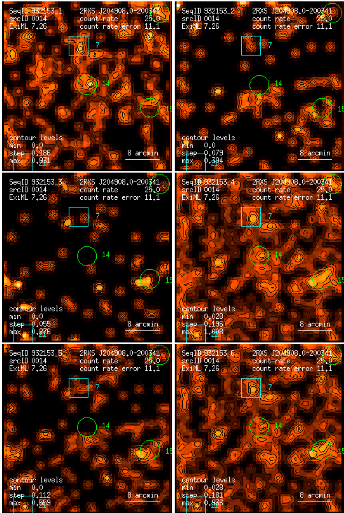
Figure 14: RASS 932153: detection 0014: band rate images, Gaussian filter: (1) PSPC channels 11 – 41, (2) 52 – 90, (3) 91 – 201, (4) 11 – 235, (5) 52 – 201, (6) 11 – 201. Broad band rates in counts/ks. Band rate contour levels in counts/ks/arcmin 2 .
