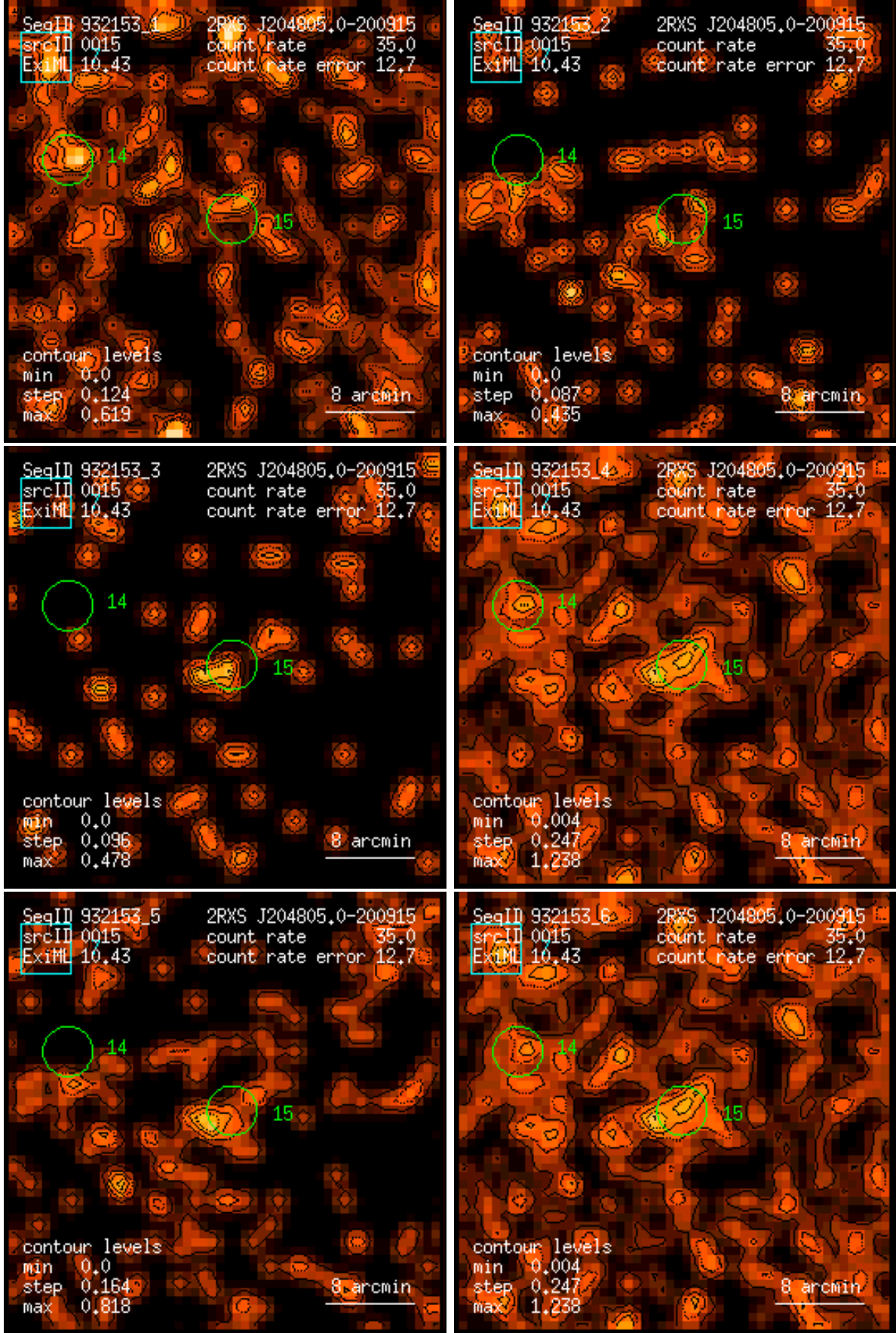
Figure 15: RASS 932153: detection 0015: band rate images, Gaussian filter: (1) PSPC channels 11 – 41, (2) 52 – 90, (3) 91 – 201, (4) 11 – 235, (5) 52 – 201, (6) 11 – 201. Broad band rates in counts/ks. Band rate contour levels in counts/ks/arcmin 2 .
