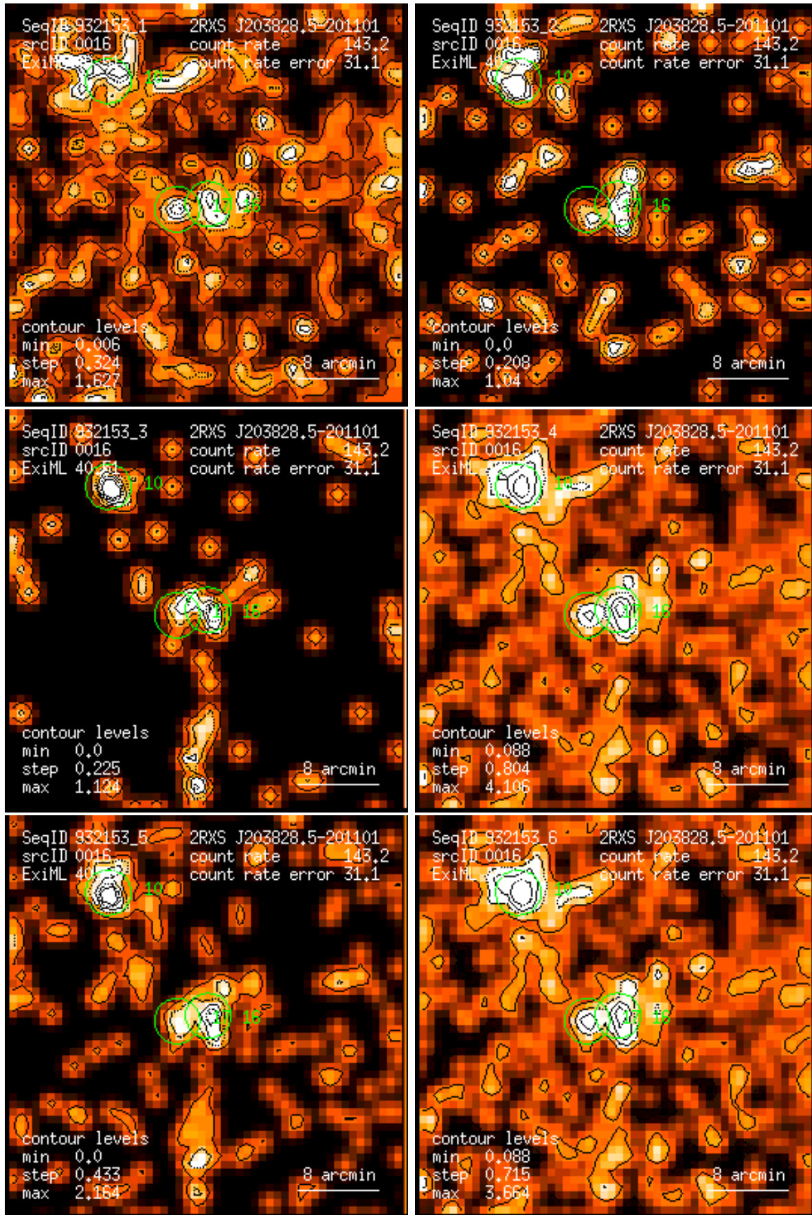
Figure 16: RASS 932153: detection 0016: band rate images, Gaussian filter: (1) PSPC channels 11 – 41, (2) 52 – 90, (3) 91 – 201, (4) 11 – 235, (5) 52 – 201, (6) 11 – 201. Broad band rates in counts/ks. Band rate contour levels in counts/ks/arcmin 2 .
