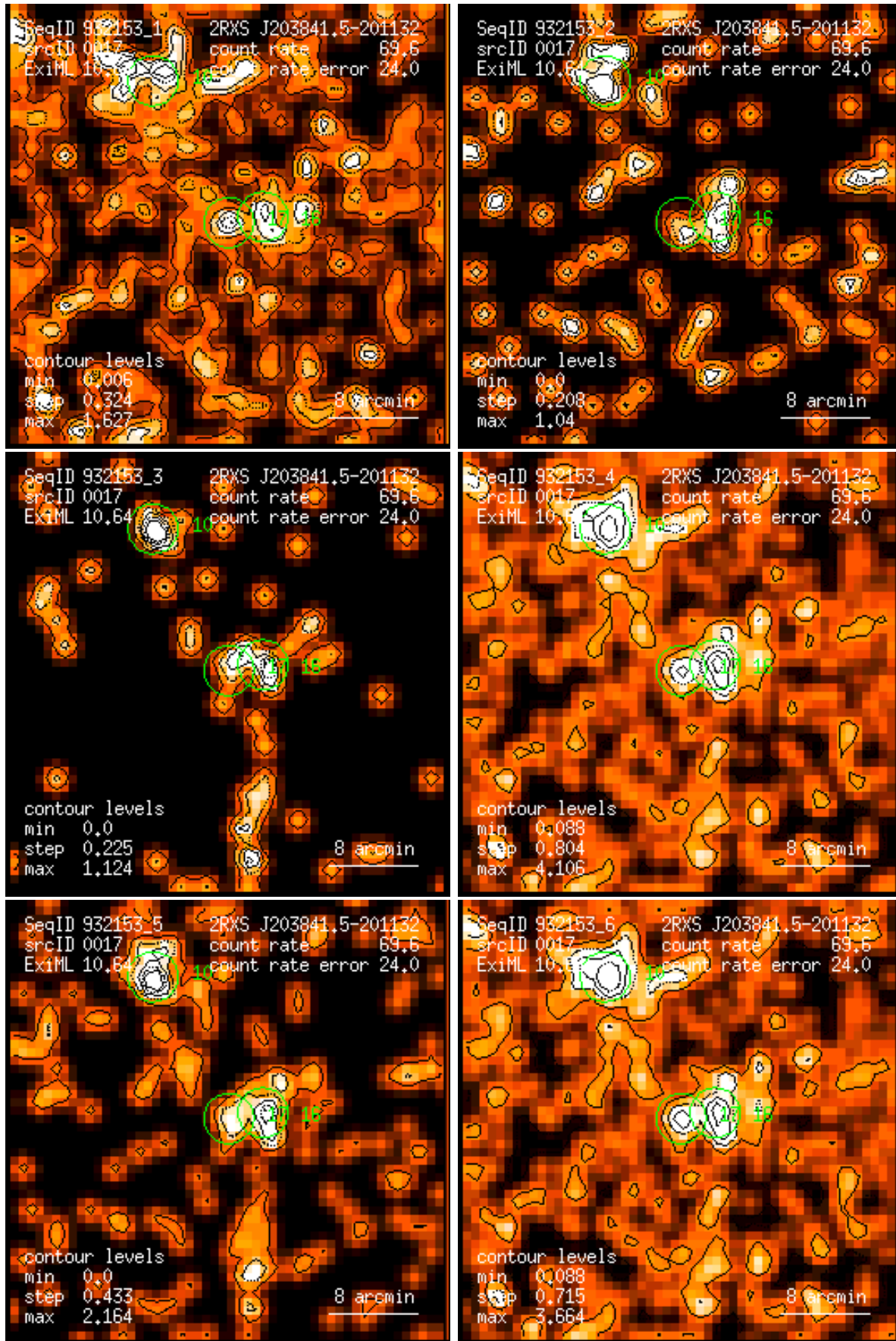
Figure 17: RASS 932153: detection 0017: band rate images, Gaussian filter: (1) PSPC channels 11 – 41, (2) 52 – 90, (3) 91 – 201, (4) 11 – 235, (5) 52 – 201, (6) 11 – 201. Broad band rates in counts/ks. Band rate contour levels in counts/ks/arcmin 2 .
