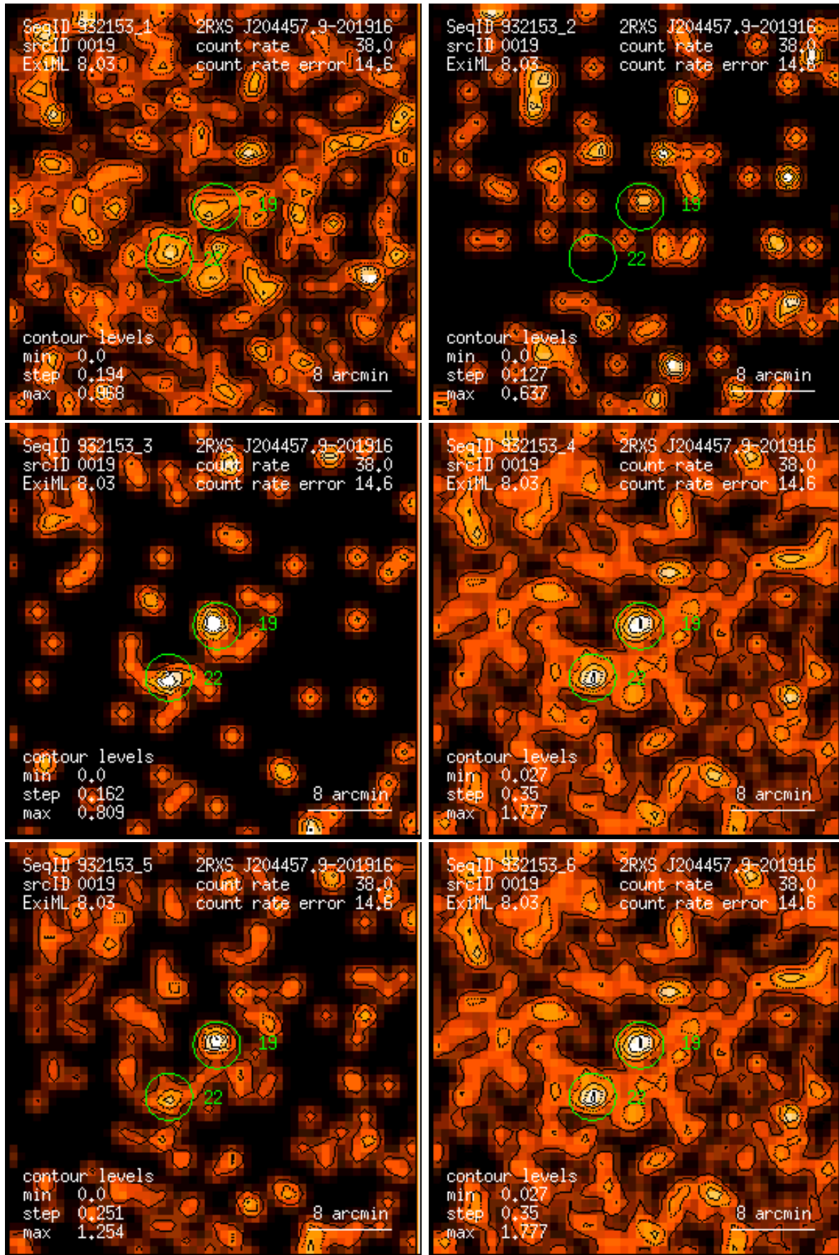
Figure 19: RASS 932153: detection 0019: band rate images, Gaussian filter: (1) PSPC channels 11 – 41, (2) 52 – 90, (3) 91 – 201, (4) 11 – 235, (5) 52 – 201, (6) 11 – 201. Broad band rates in counts/ks. Band rate contour levels in counts/ks/arcmin 2 .
