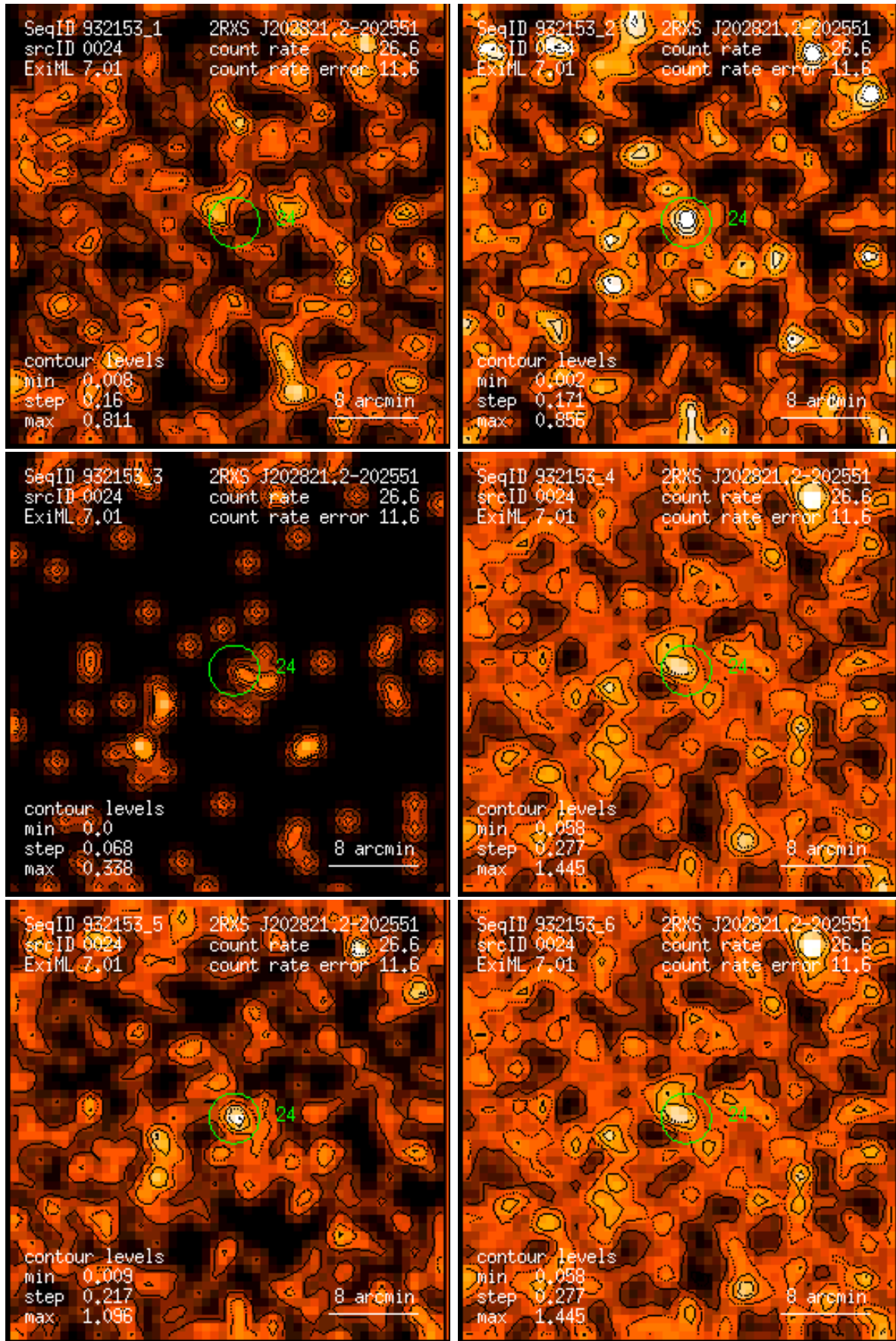
Figure 24: RASS 932153: detection 0024: band rate images, Gaussian filter: (1) PSPC channels 11 – 41, (2) 52 – 90, (3) 91 – 201, (4) 11 – 235, (5) 52 – 201, (6) 11 – 201. Broad band rates in counts/ks. Band rate contour levels in counts/ks/arcmin 2 .
