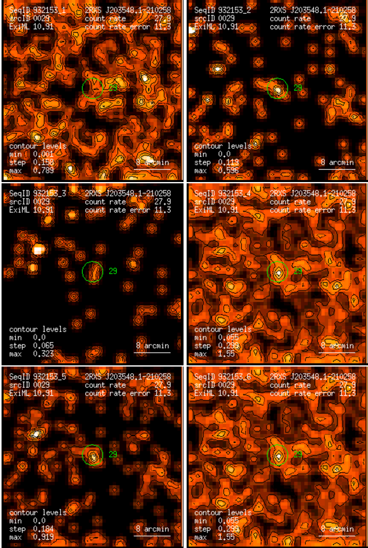
Figure 29: RASS 932153: detection 0029: band rate images, Gaussian filter: (1) PSPC channels 11 – 41, (2) 52 – 90, (3) 91 – 201, (4) 11 – 235, (5) 52 – 201, (6) 11 – 201. Broad band rates in counts/ks. Band rate contour levels in counts/ks/arcmin 2 .
