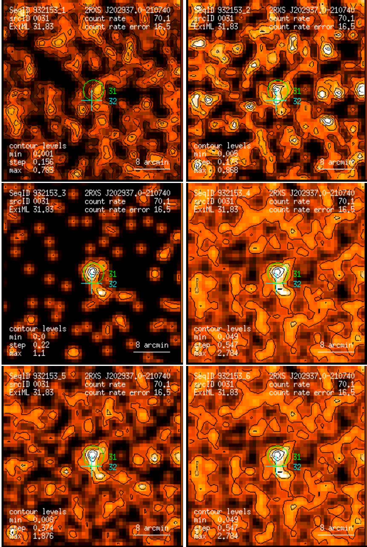
Figure 31: RASS 932153: detection 0031: band rate images, Gaussian filter: (1) PSPC channels 11 – 41, (2) 52 – 90, (3) 91 – 201, (4) 11 – 235, (5) 52 – 201, (6) 11 – 201. Broad band rates in counts/ks. Band rate contour levels in counts/ks/arcmin 2 .
