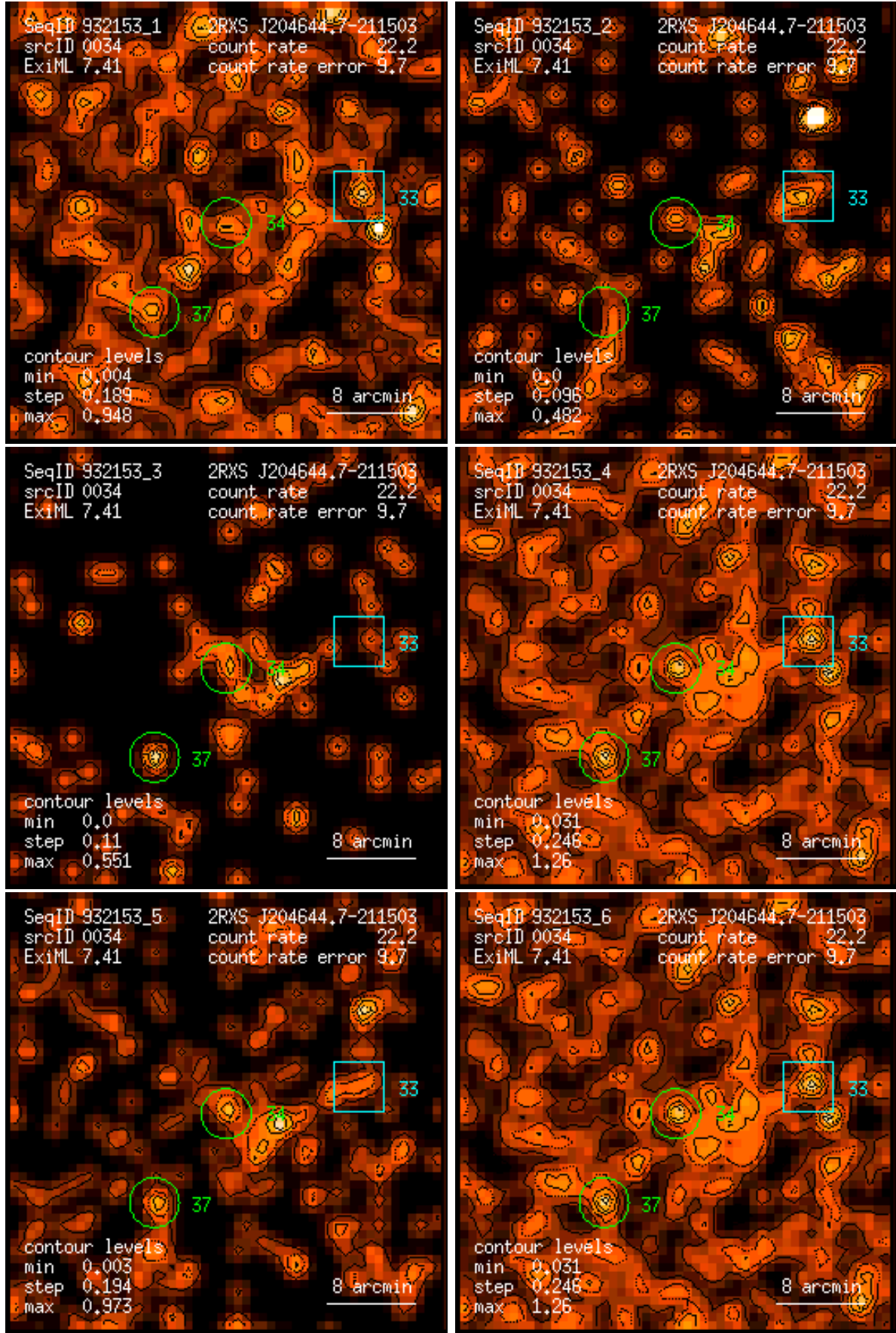
Figure 34: RASS 932153: detection 0034: band rate images, Gaussian filter: (1) PSPC channels 11 – 41, (2) 52 – 90, (3) 91 – 201, (4) 11 – 235, (5) 52 – 201, (6) 11 – 201. Broad band rates in counts/ks. Band rate contour levels in counts/ks/arcmin 2 .
