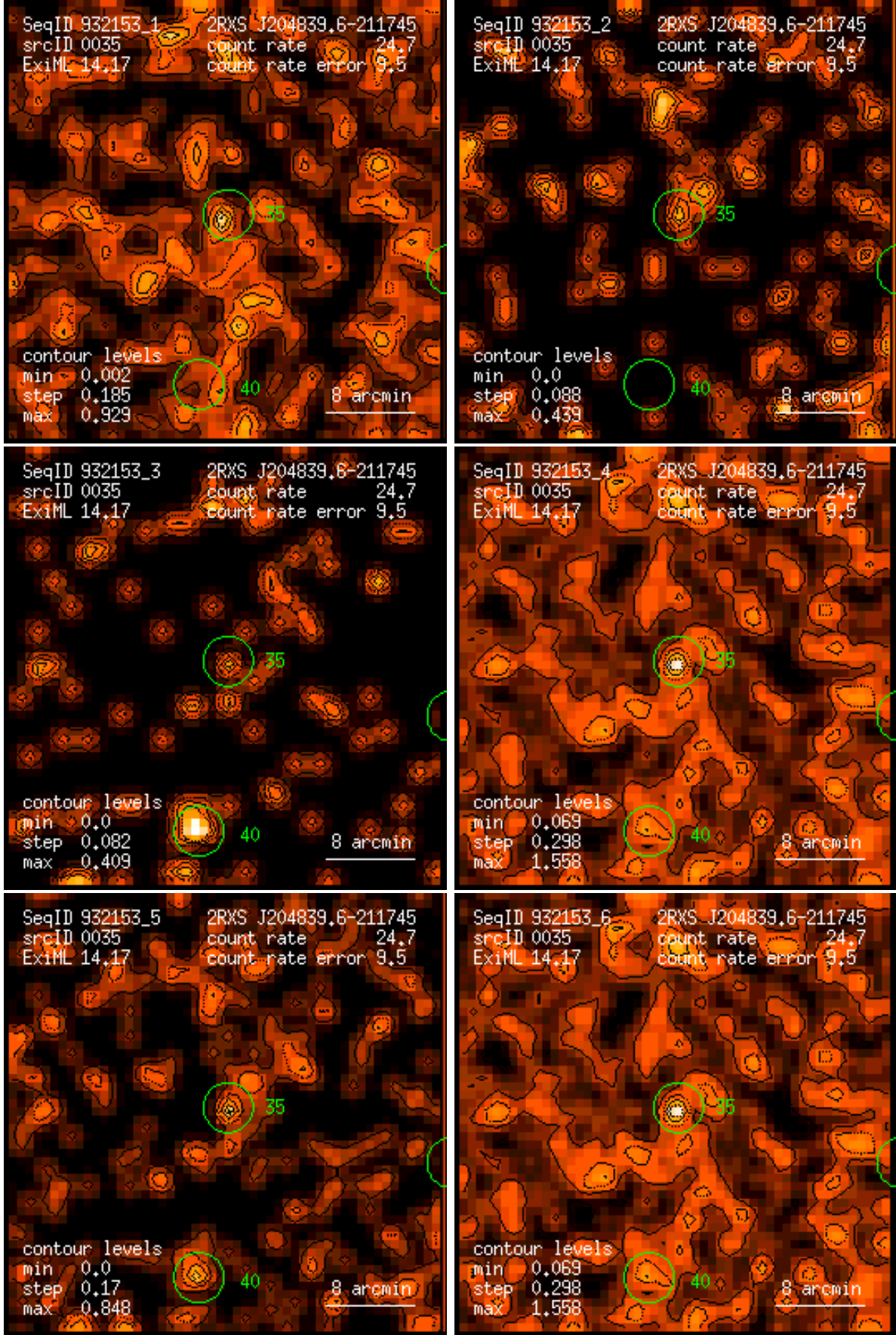
Figure 35: RASS 932153: detection 0035: band rate images, Gaussian filter: (1) PSPC channels 11 – 41, (2) 52 – 90, (3) 91 – 201, (4) 11 – 235, (5) 52 – 201, (6) 11 – 201. Broad band rates in counts/ks. Band rate contour levels in counts/ks/arcmin 2 .
