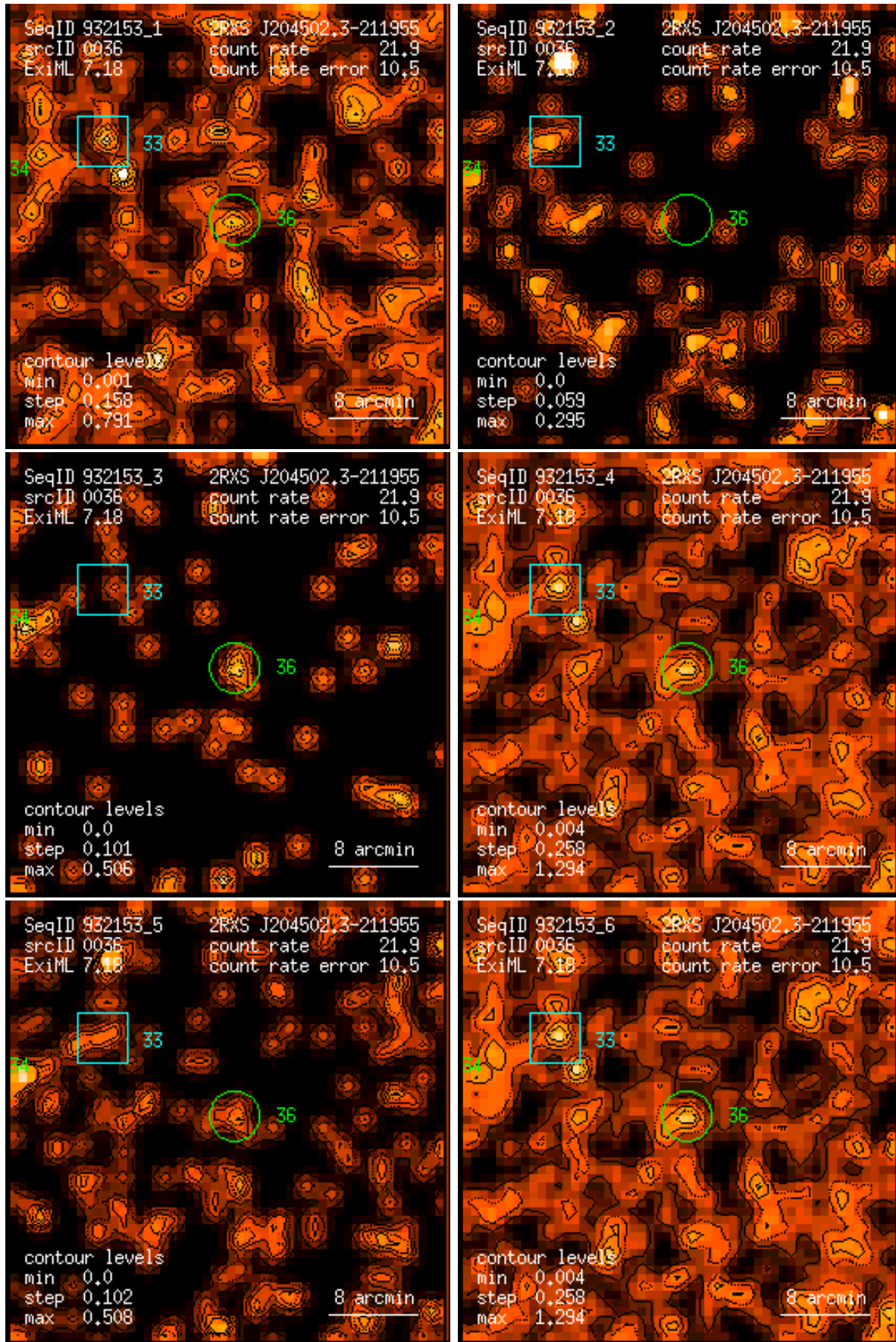
Figure 36: RASS 932153: detection 0036: band rate images, Gaussian filter: (1) PSPC channels 11 – 41, (2) 52 – 90, (3) 91 – 201, (4) 11 – 235, (5) 52 – 201, (6) 11 – 201. Broad band rates in counts/ks. Band rate contour levels in counts/ks/arcmin 2 .
