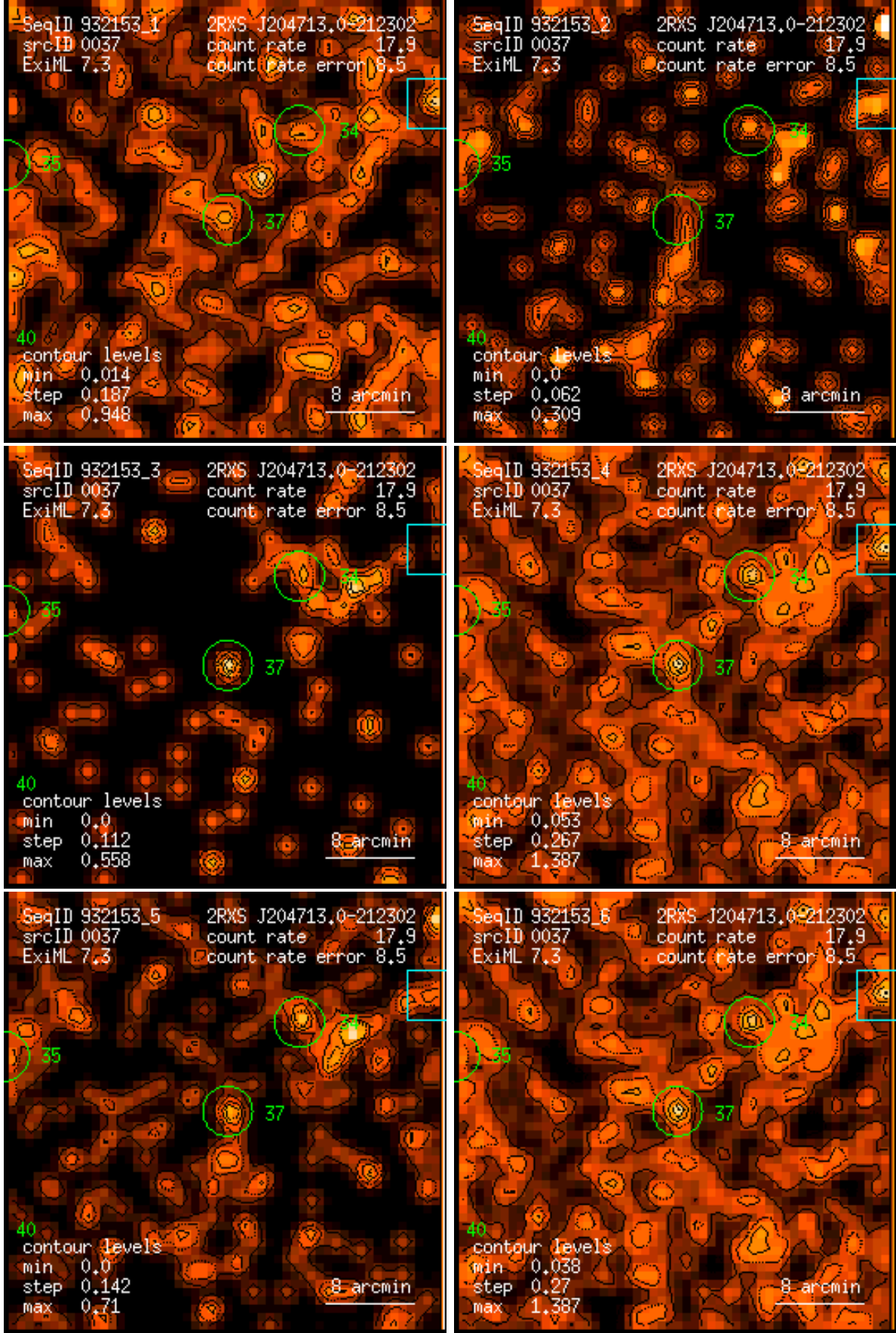
Figure 37: RASS 932153: detection 0037: band rate images, Gaussian filter: (1) PSPC channels 11 – 41, (2) 52 – 90, (3) 91 – 201, (4) 11 – 235, (5) 52 – 201, (6) 11 – 201. Broad band rates in counts/ks. Band rate contour levels in counts/ks/arcmin 2 .
