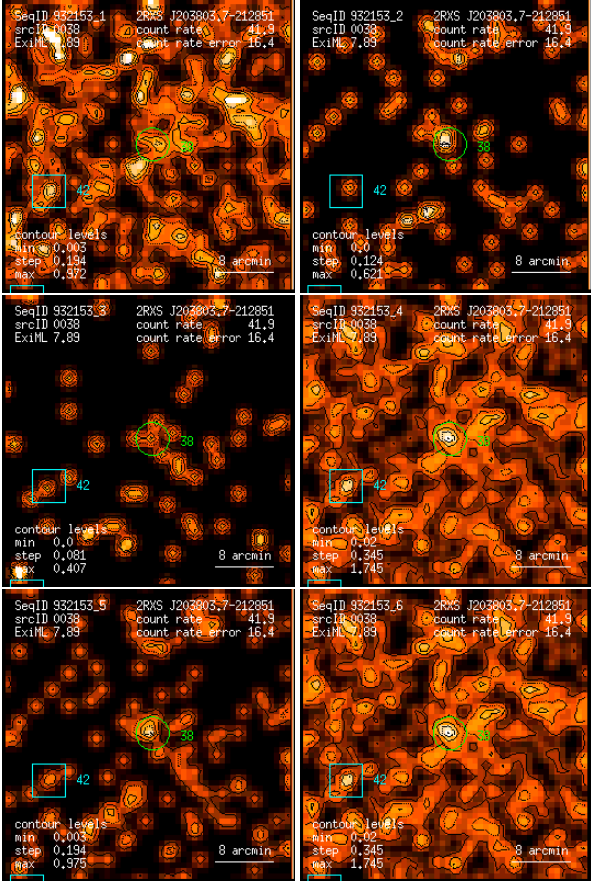
Figure 38: RASS 932153: detection 0038: band rate images, Gaussian filter: (1) PSPC channels 11 – 41, (2) 52 – 90, (3) 91 – 201, (4) 11 – 235, (5) 52 – 201, (6) 11 – 201. Broad band rates in counts/ks. Band rate contour levels in counts/ks/arcmin 2 .
