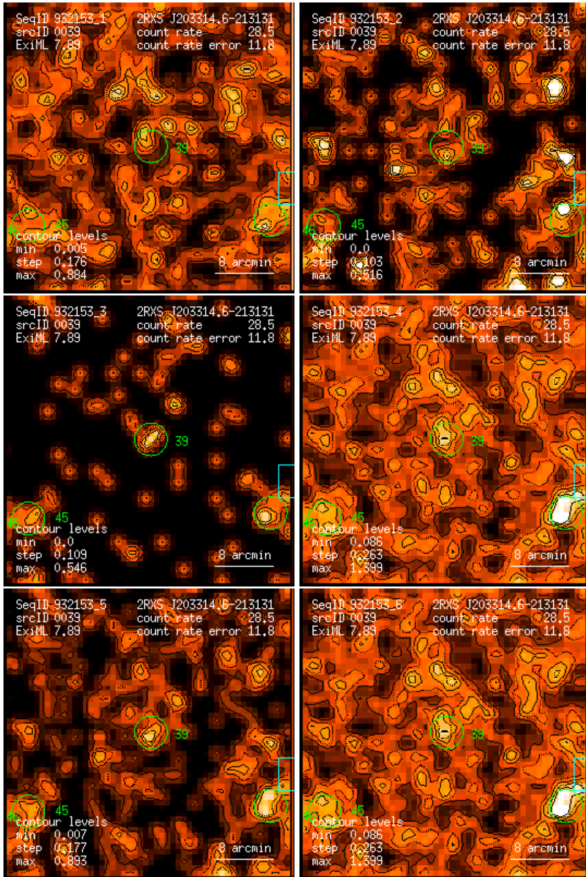
Figure 39: RASS 932153: detection 0039: band rate images, Gaussian filter: (1) PSPC channels 11 – 41, (2) 52 – 90, (3) 91 – 201, (4) 11 – 235, (5) 52 – 201, (6) 11 – 201. Broad band rates in counts/ks. Band rate contour levels in counts/ks/arcmin 2 .
