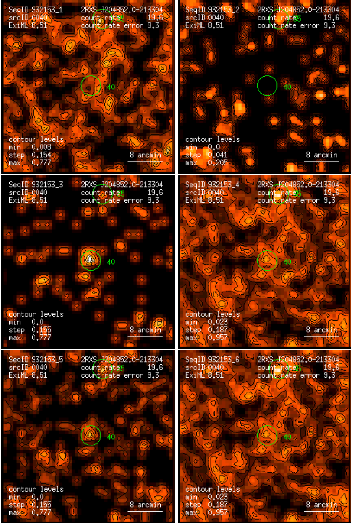
Figure 40: RASS 932153: detection 0040: band rate images, Gaussian filter: (1) PSPC channels 11 – 41, (2) 52 – 90, (3) 91 – 201, (4) 11 – 235, (5) 52 – 201, (6) 11 – 201. Broad band rates in counts/ks. Band rate contour levels in counts/ks/arcmin 2 .
