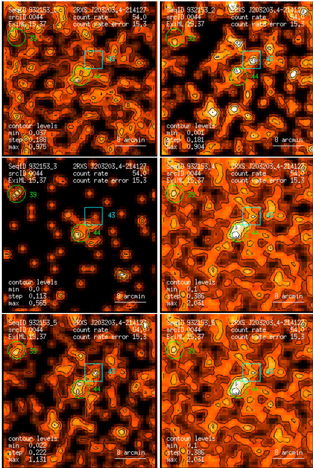
Figure 44: RASS 932153: detection 0044: band rate images, Gaussian filter: (1) PSPC channels 11 – 41, (2) 52 – 90, (3) 91 – 201, (4) 11 – 235, (5) 52 – 201, (6) 11 – 201. Broad band rates in counts/ks. Band rate contour levels in counts/ks/arcmin 2 .
