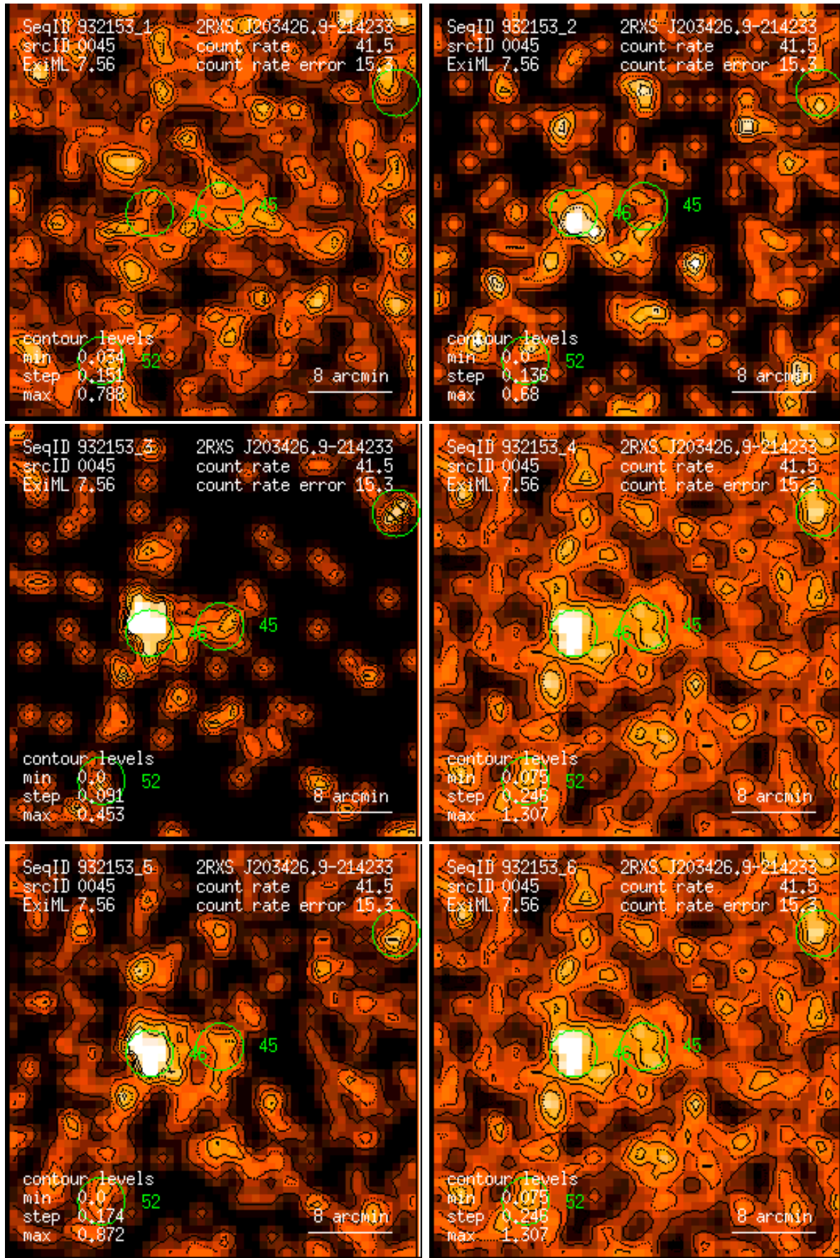
Figure 45: RASS 932153: detection 0045: band rate images, Gaussian filter: (1) PSPC channels 11 – 41, (2) 52 – 90, (3) 91 – 201, (4) 11 – 235, (5) 52 – 201, (6) 11 – 201. Broad band rates in counts/ks. Band rate contour levels in counts/ks/arcmin 2 .
